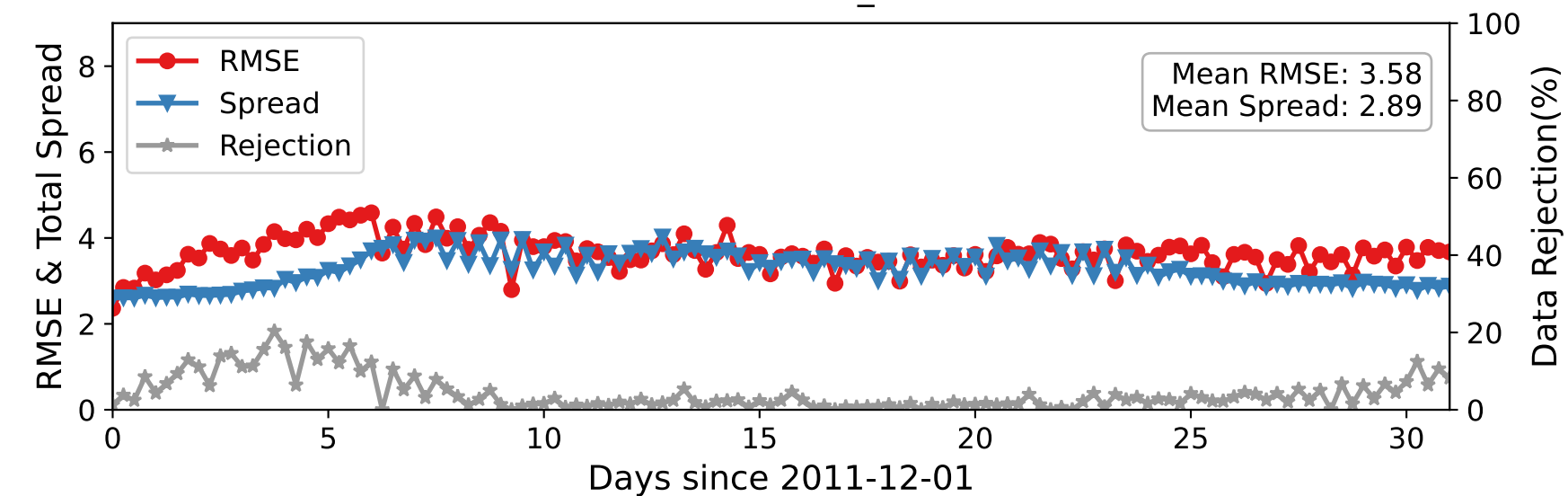
DARTEN20 — RADIOSONDE_U at 350-450 hPa
