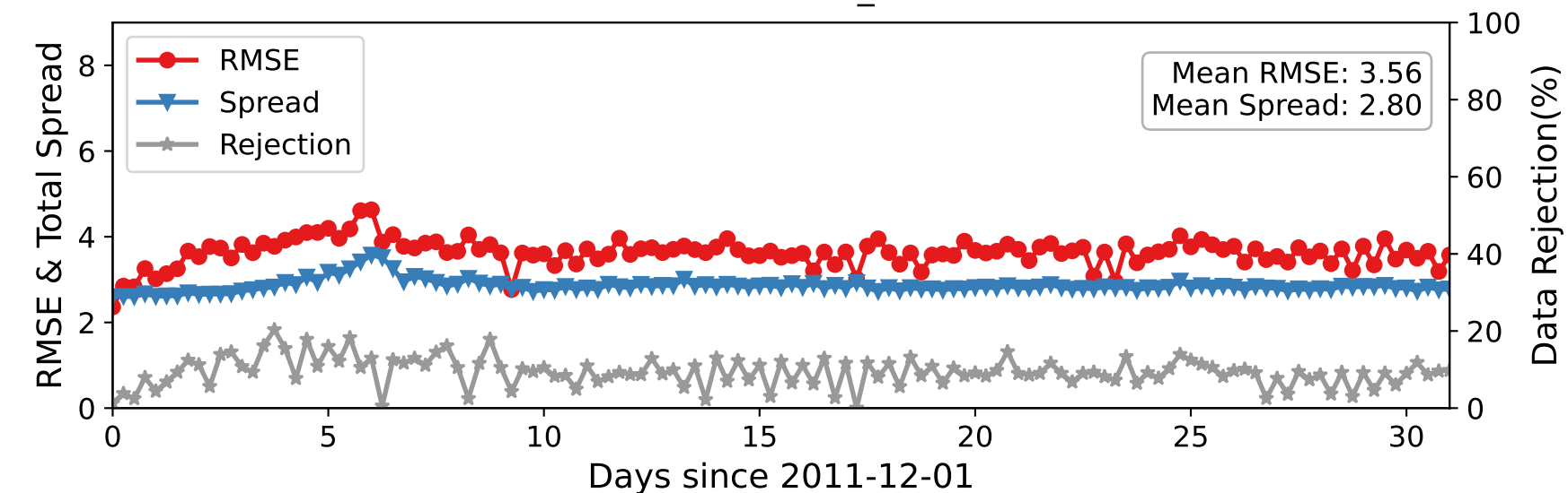
DARTEN40 — RADIOSONDE_U at 350-450 hPa
