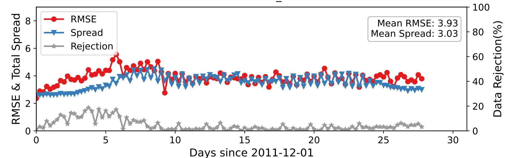
DARTEN10 — RADIOSONDE_U at 350-450 hPa
