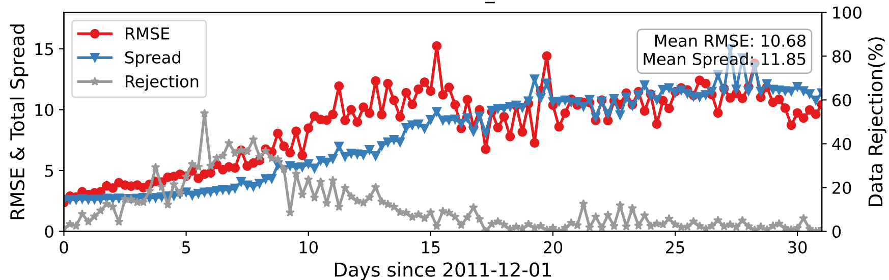
CTRLN10 — RADIOSONDE_U at 350-450 hPa
