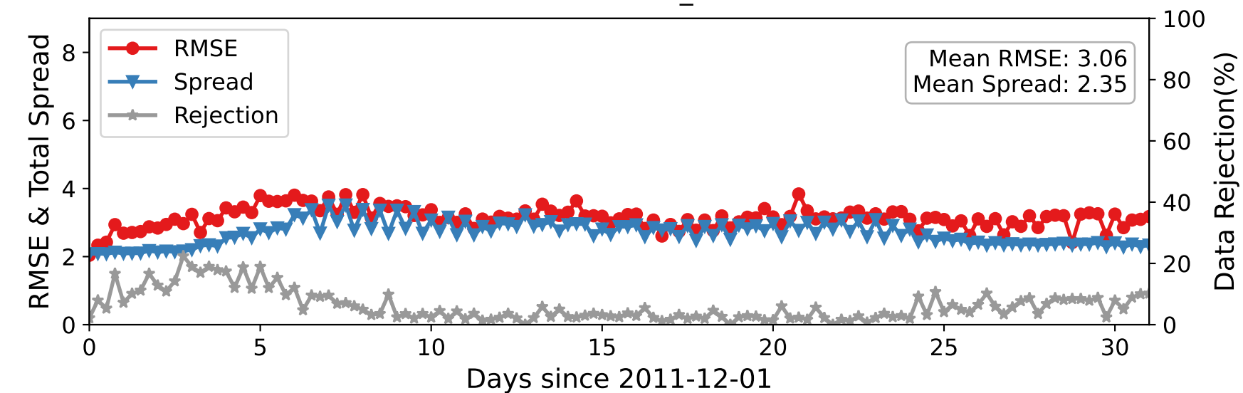
DARTEN20 — RADIOSONDE_U at 450-600 hPa
