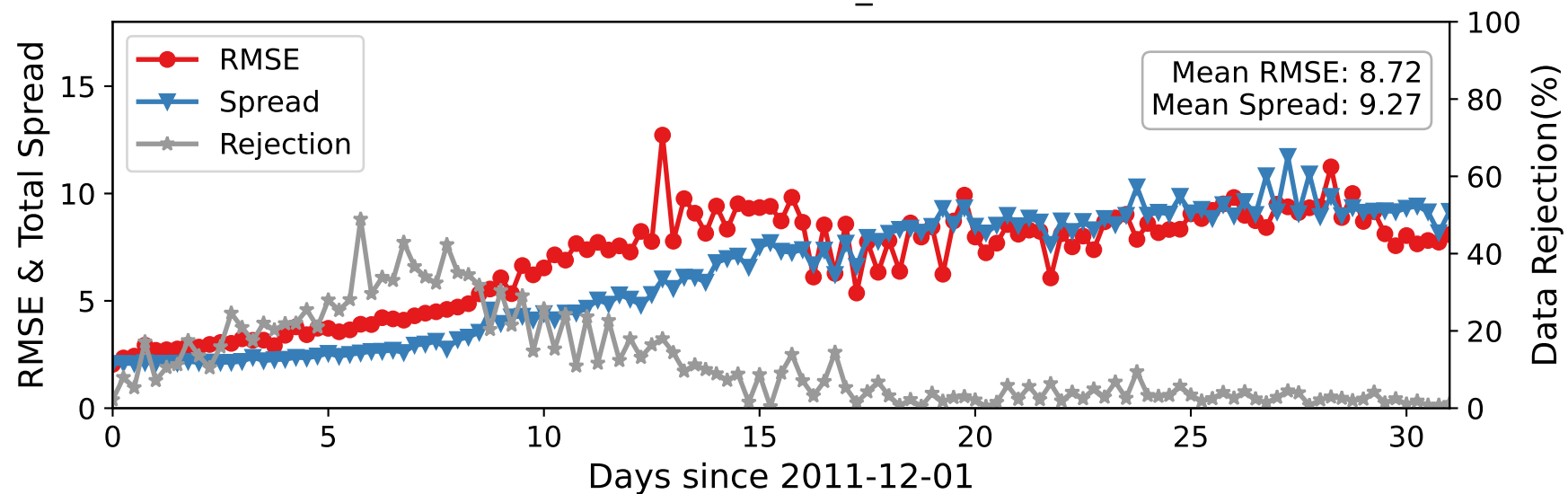
CTRLN10 — RADIOSONDE_U at 450-600 hPa
