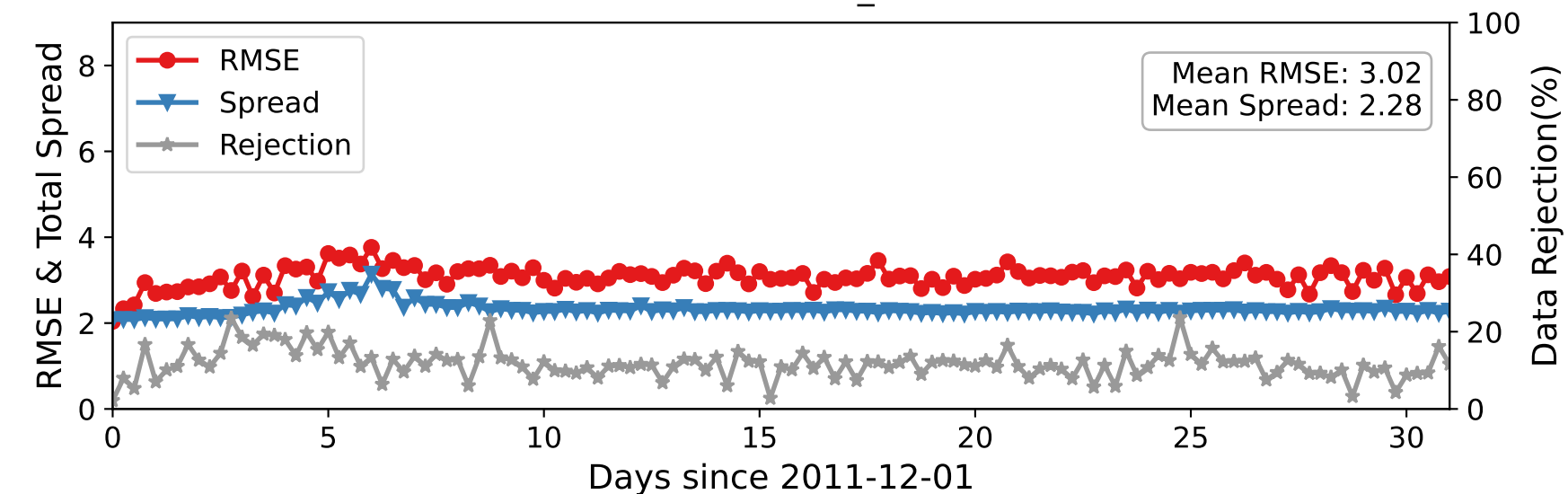
DARTEN40 — RADIOSONDE_U at 450-600 hPa
