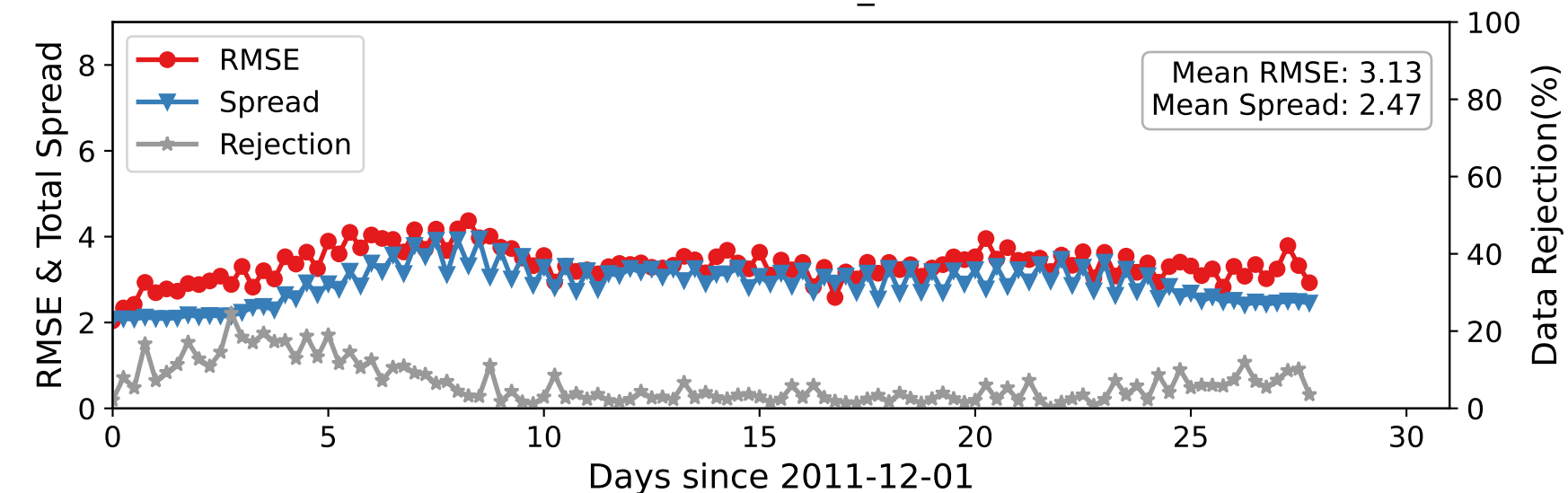
DARTEN10 — RADIOSONDE_U at 450-600 hPa
