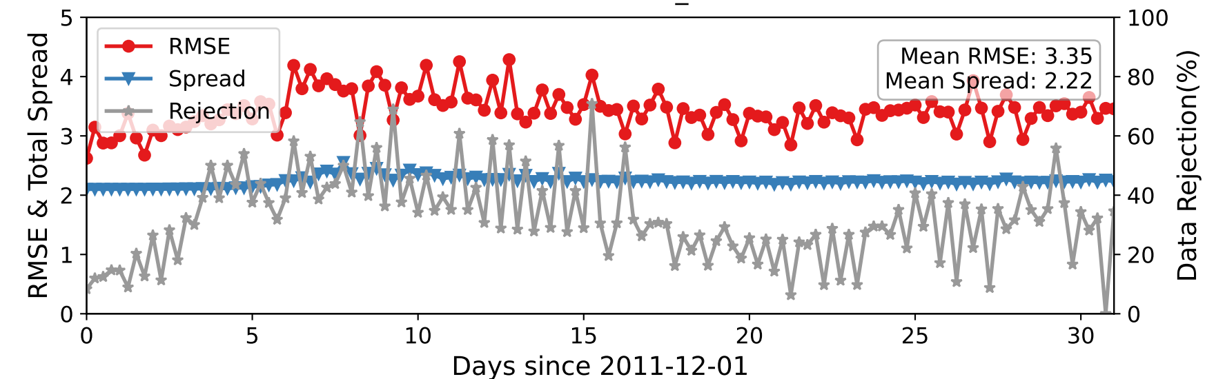
DARTEN40 — RADIOSONDE_U at 15-35 hPa
