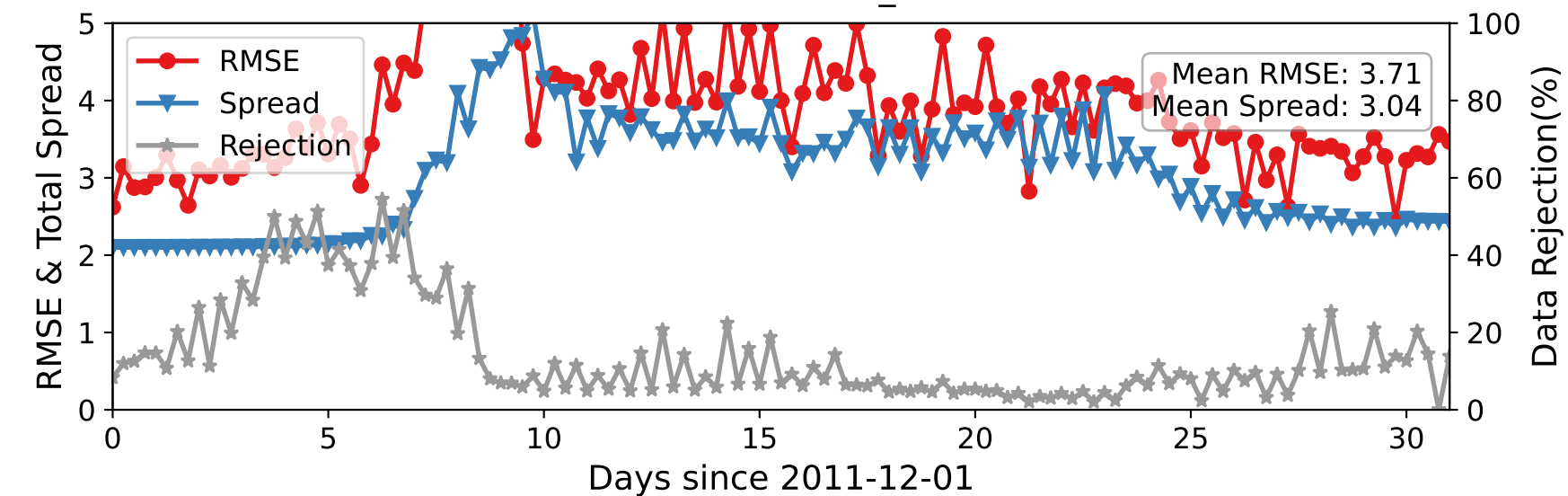
DARTEN20 — RADIOSONDE_U at 15-35 hPa
