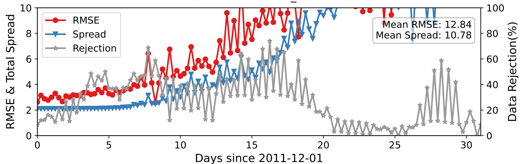
CTRLLEN10 — RADIOSONDE_U at 15-35 hPa
