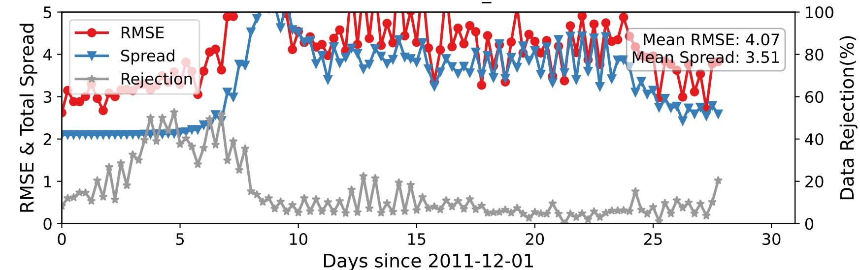
DARTEN10 — RADIOSONDE_U at 15-35 hPa
