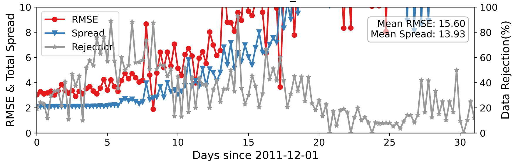
CTRLN10 — RADIOSONDE_U at 2-15 hPa
