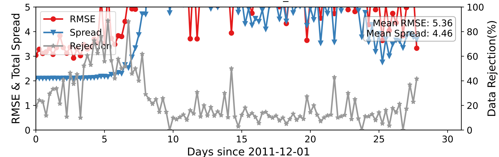
DARTEN10 — RADIOSONDE_U at 2-15 hPa
