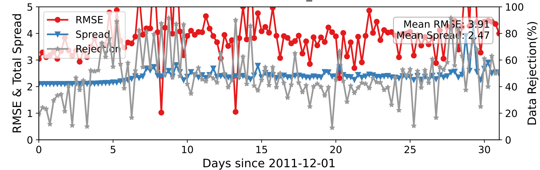
DARTEN40 — RADIOSONDE_U at 2-15 hPa
