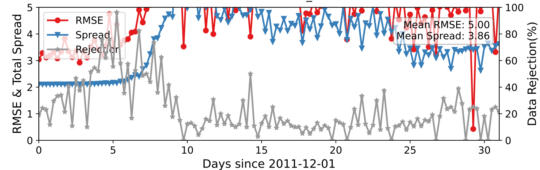
DARTEN20 — RADIOSONDE_U at 2-15 hPa
