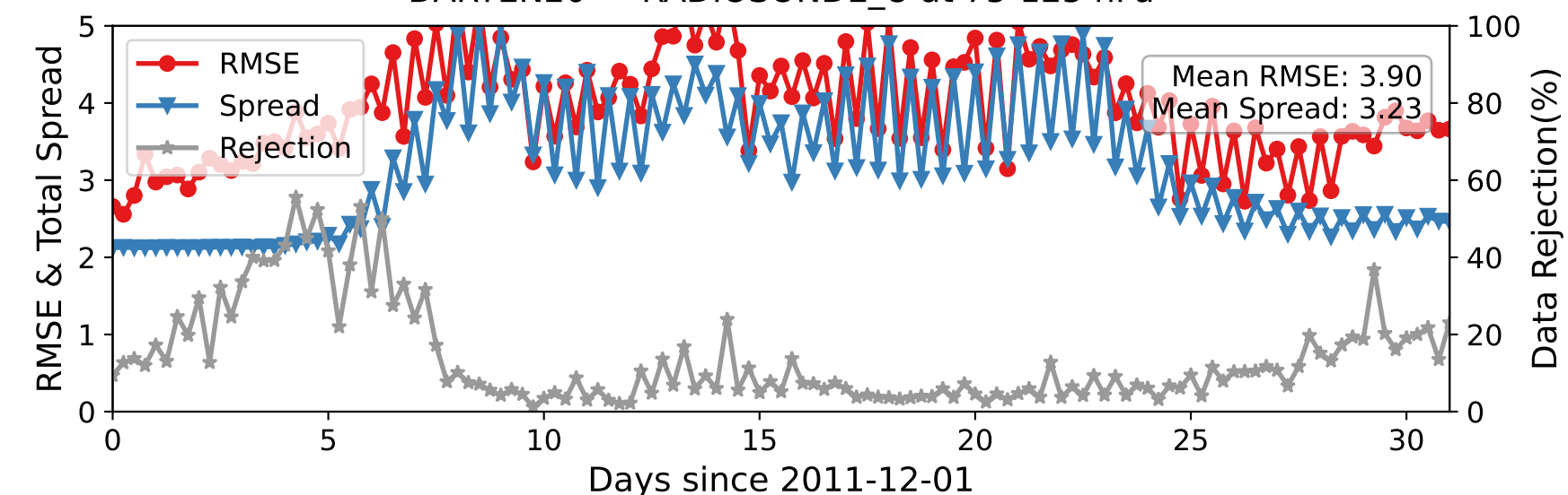
DARTEN20 — RADIOSONDE_U at 75-125 hPa
