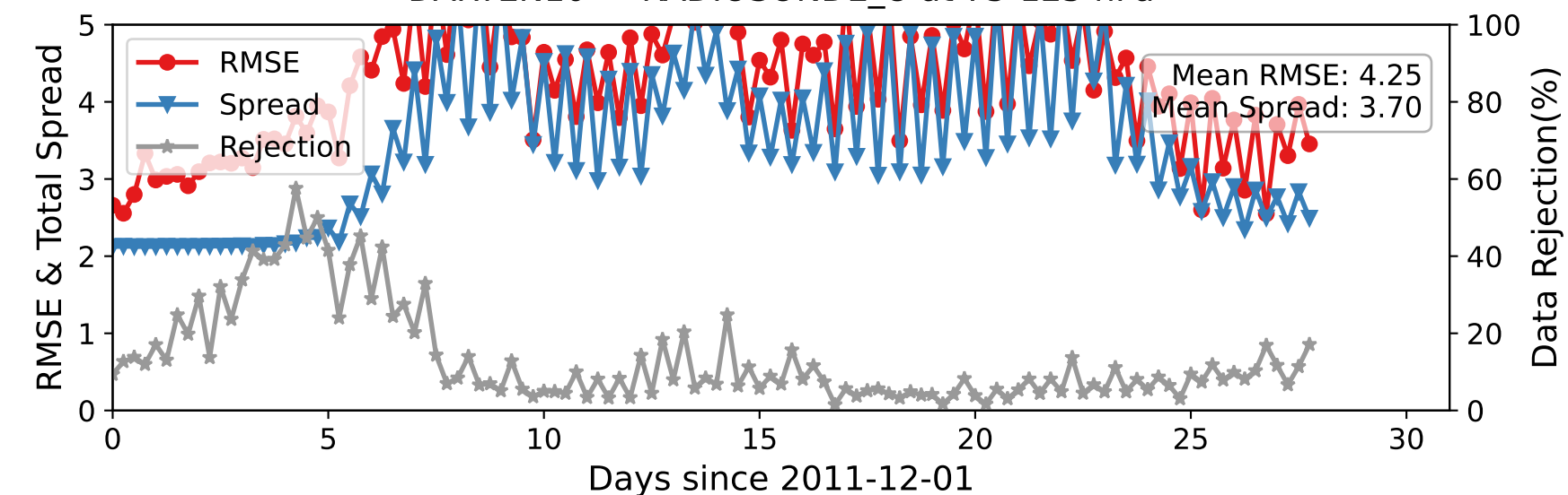
DARTEN10 — RADIOSONDE_U at 75-125 hPa
