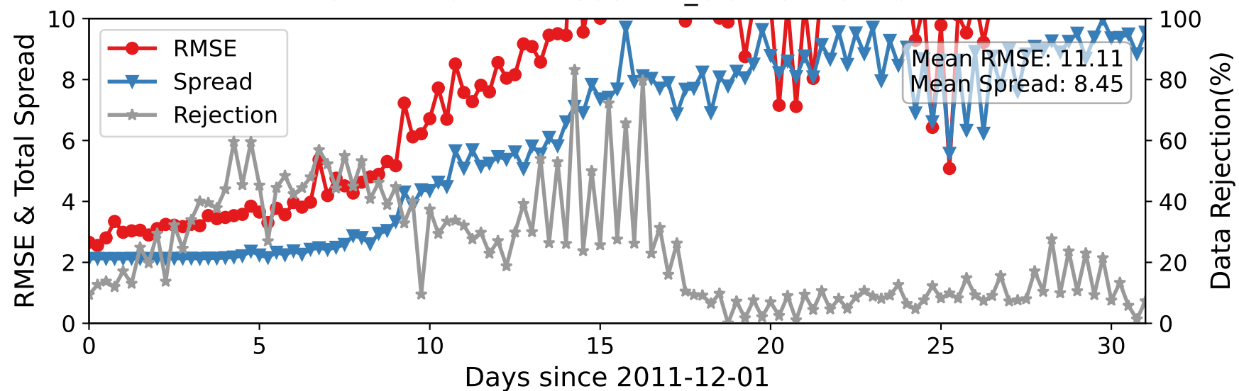
CTRLN10 — RADIOSONDE_U at 75-125 hPa
