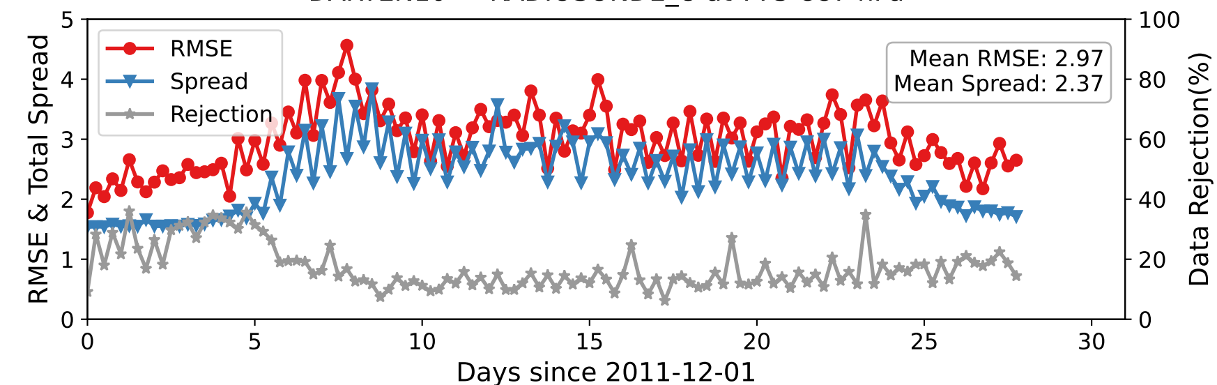
DARTEN10 — RADIOSONDE_U at 775-887 hPa
