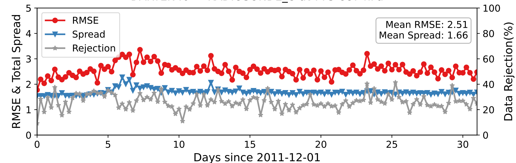
DARTEN40 — RADIOSONDE_U at 775-887 hPa
