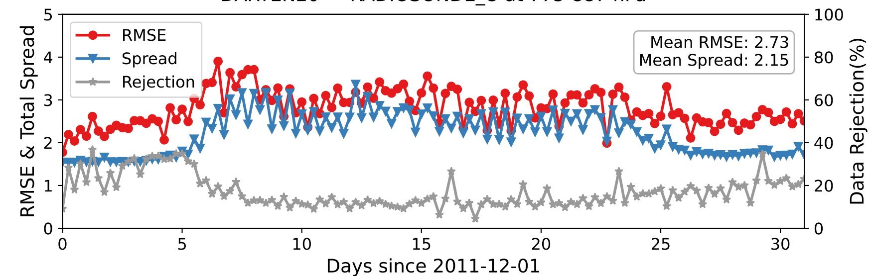
DARTEN20 — RADIOSONDE_U at 775-887 hPa
