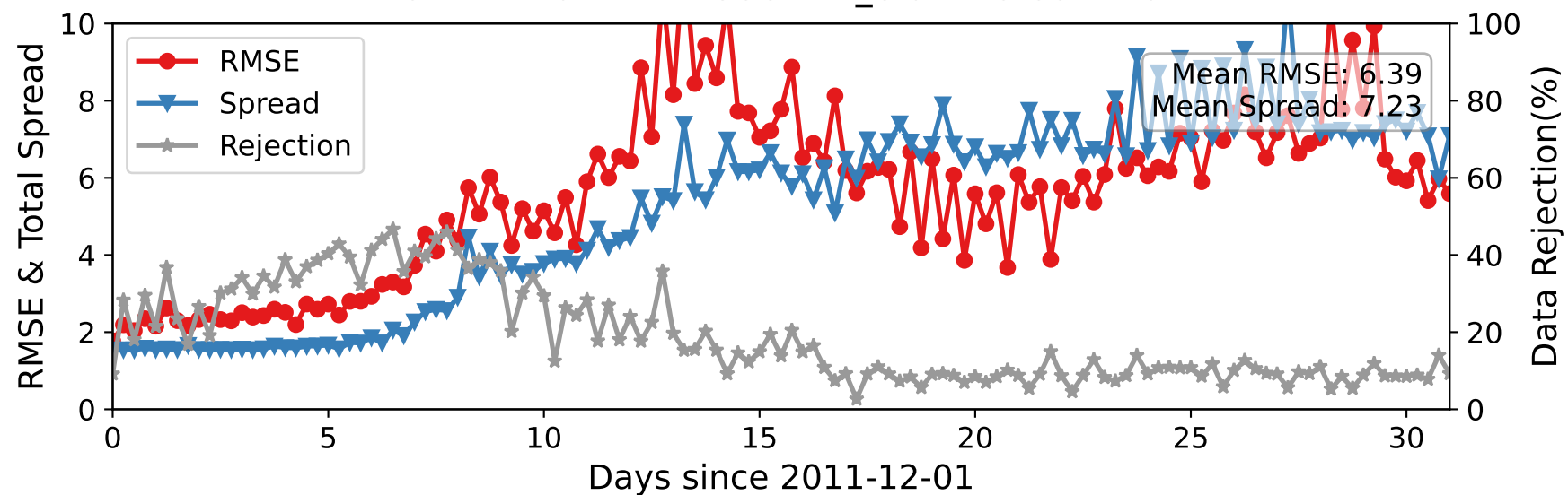
CTRLN10 — RADIOSONDE_U at 775-887 hPa
