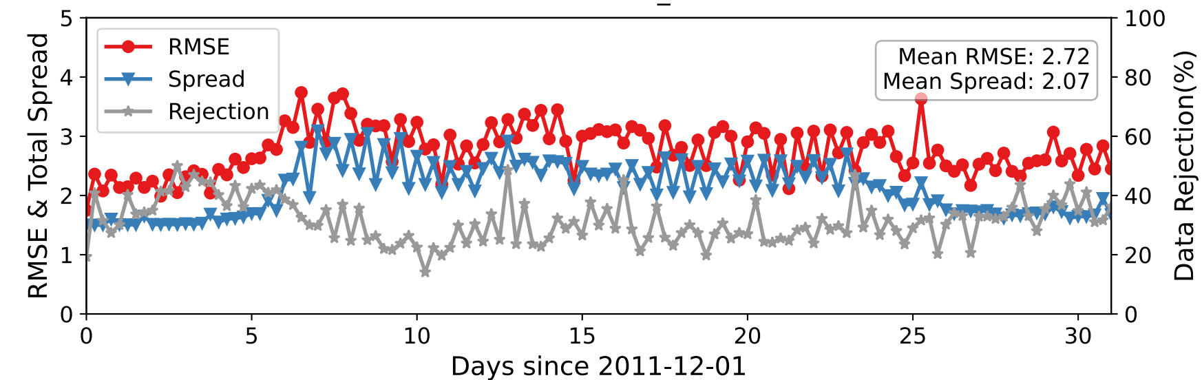
DARTEN20 — RADIOSONDE_U at 887-962 hPa
