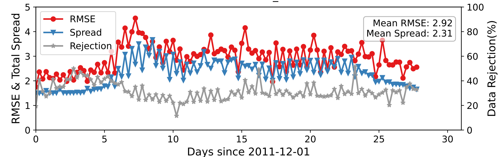
DARTEN10 — RADIOSONDE_U at 887-962 hPa
