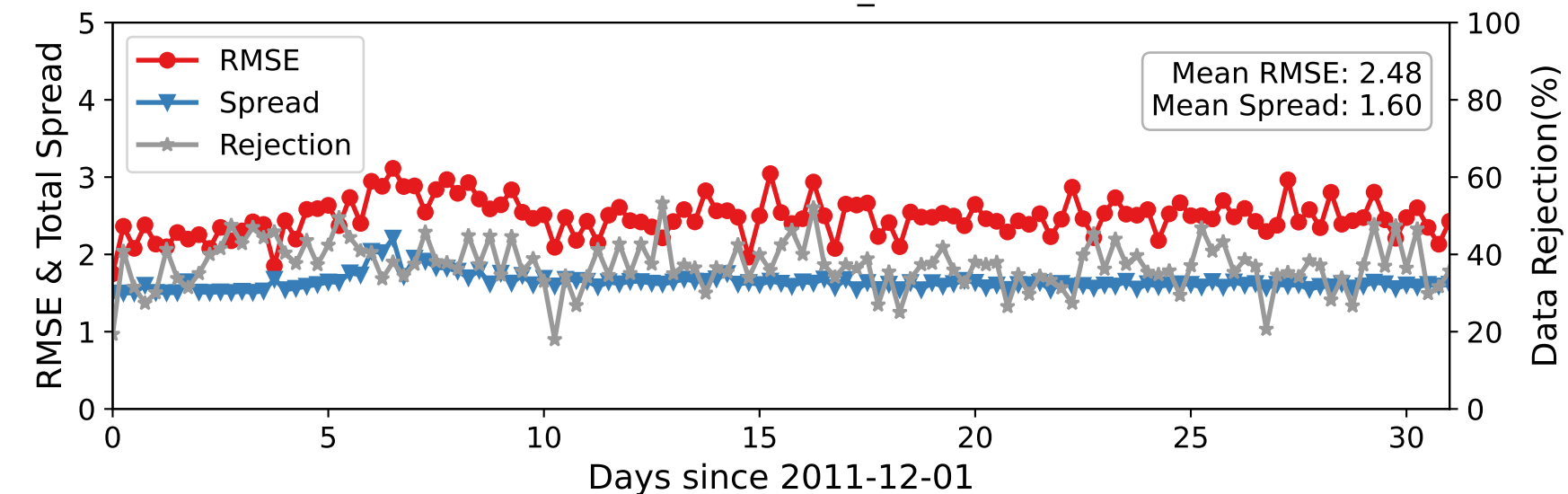
DARTEN40 — RADIOSONDE_U at 887-962 hPa
