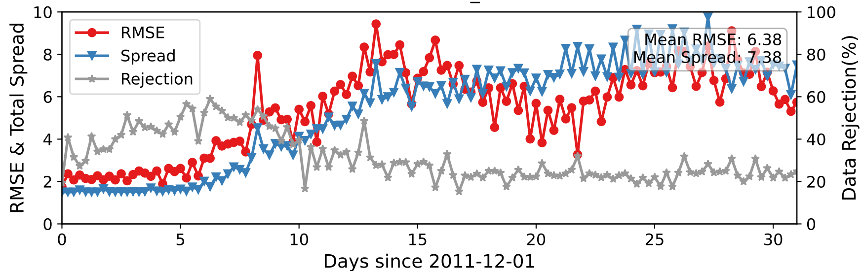
CTRLN10 — RADIOSONDE_U at 887-962 hPa
