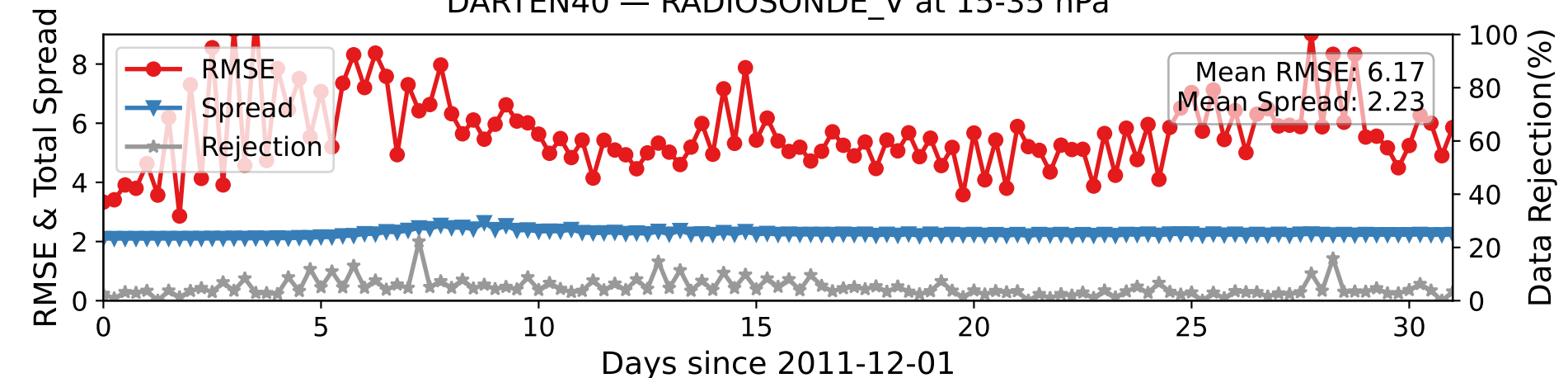
DARTEN40 — RADIOSONDE_V at 15-35 hPa
