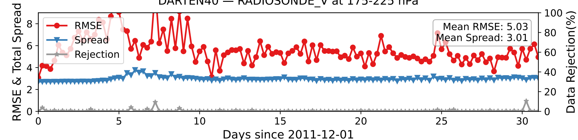
DARTEN40 — RADIOSONDE_V at 175-225 hPa
