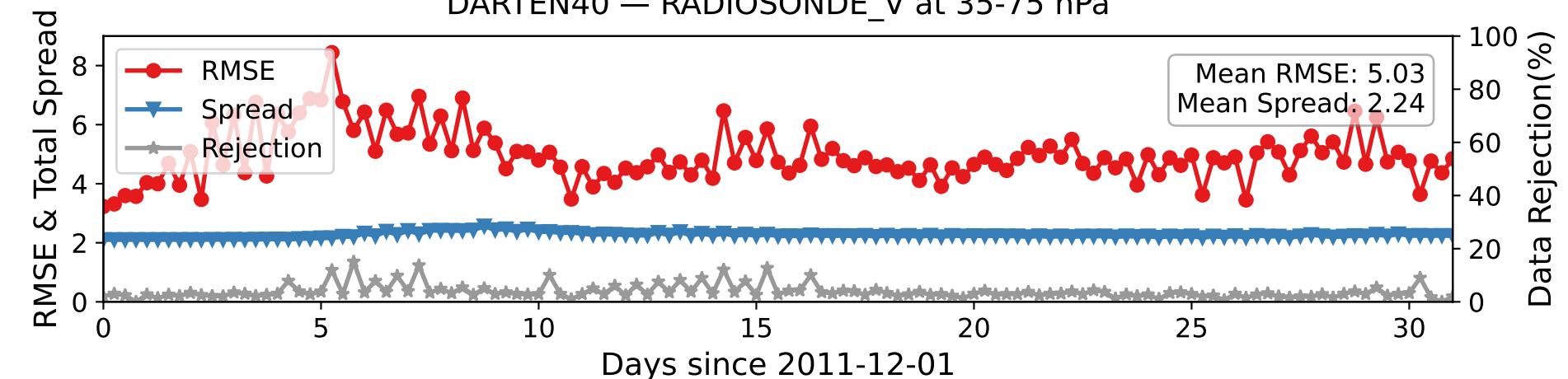
DARTEN40 — RADIOSONDE_V at 35-75 hPa
