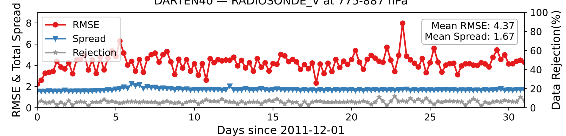
DARTEN40 — RADIOSONDE_V at 775-887 hPa
