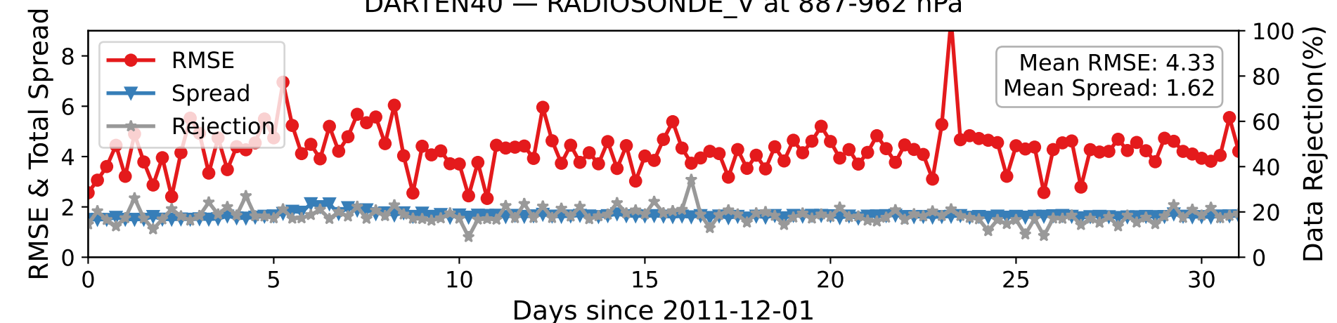
DARTEN40 — RADIOSONDE_V at 887-962 hPa
