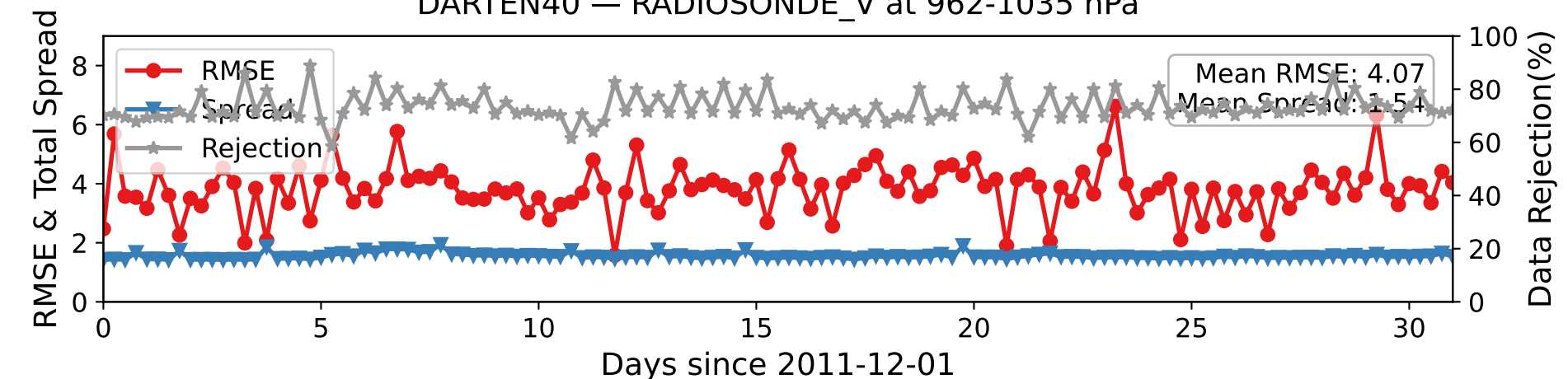
DARTEN40 — RADIOSONDE_V at 962-1035 hPa
