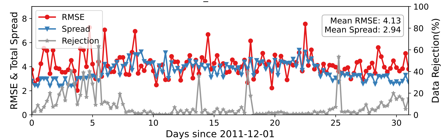
DARTEN20 — U_WIND at 125-175 hPa
