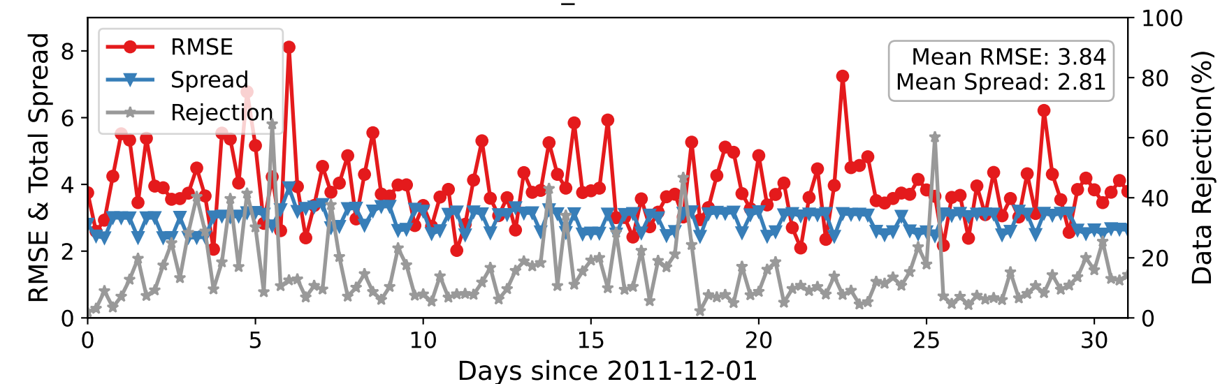
DARTEN40 — U_WIND at 125-175 hPa
