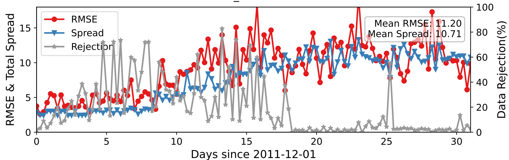
CTRLN10 — U_WIND at 125-175 hPa
