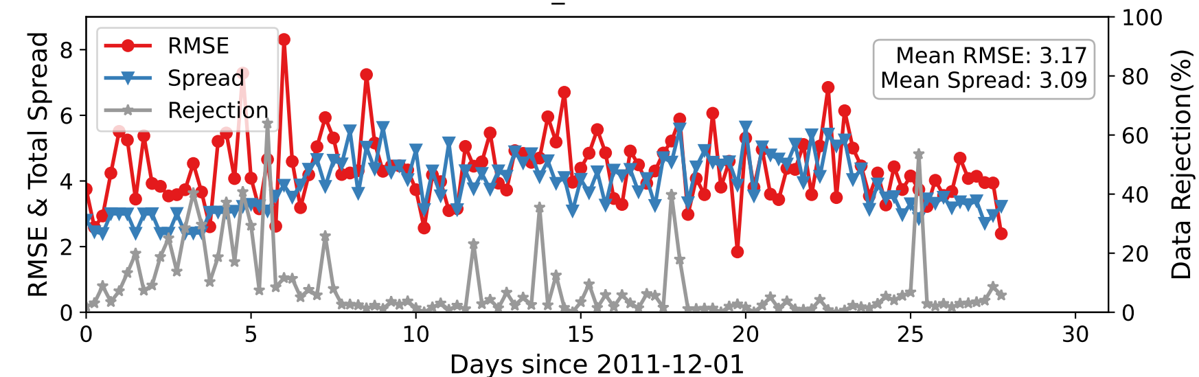
DARTEN10 — U_WIND at 125-175 hPa
