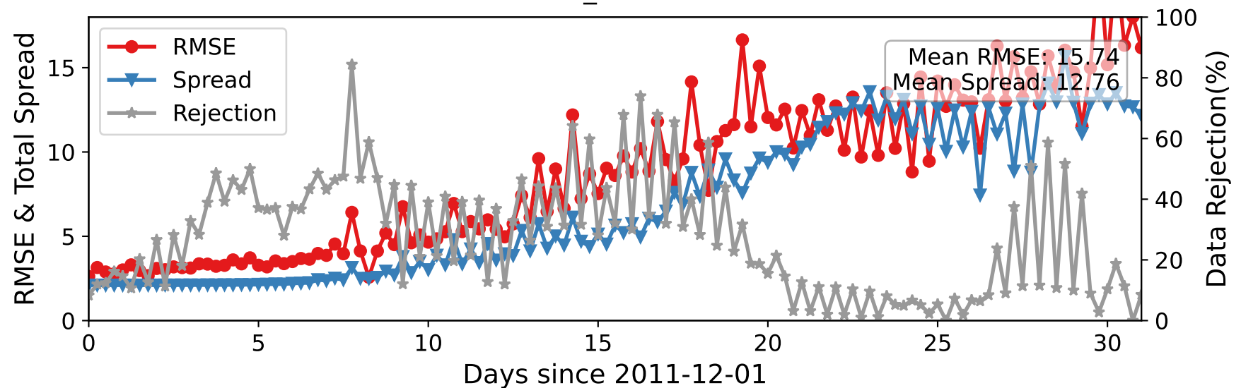
CTRLN10 — U_WIND at 15-35 hPa
