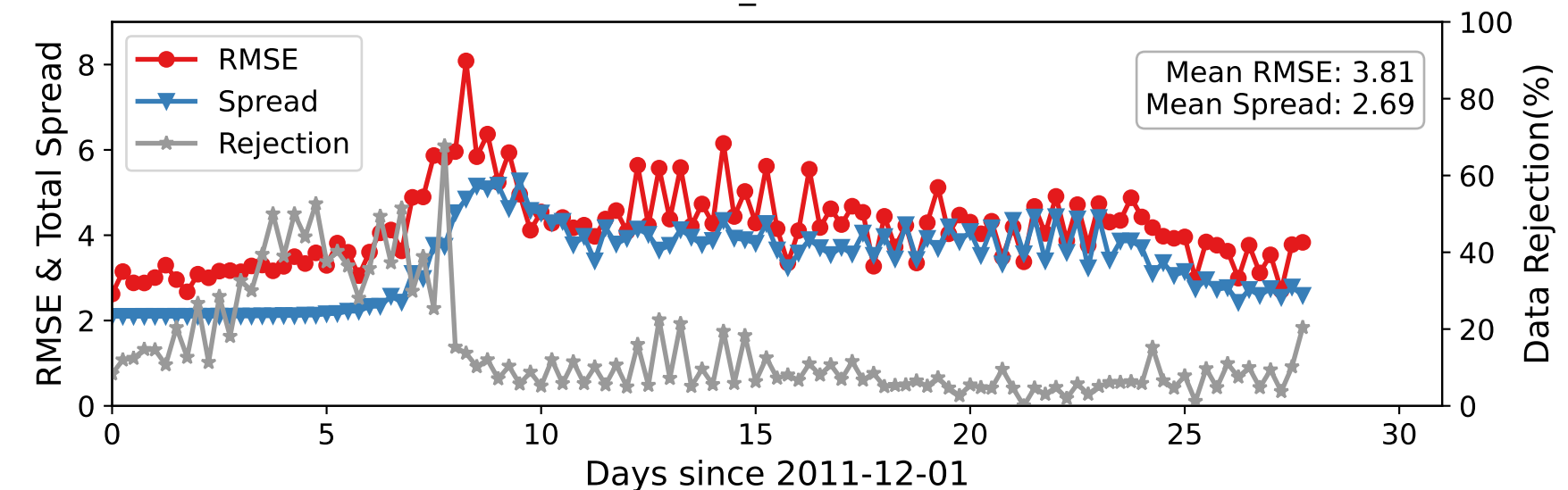
DARTEN10 — U_WIND at 15-35 hPa
