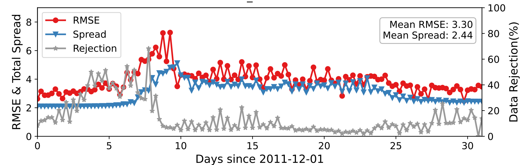
DARTEN20 — U_WIND at 15-35 hPa
