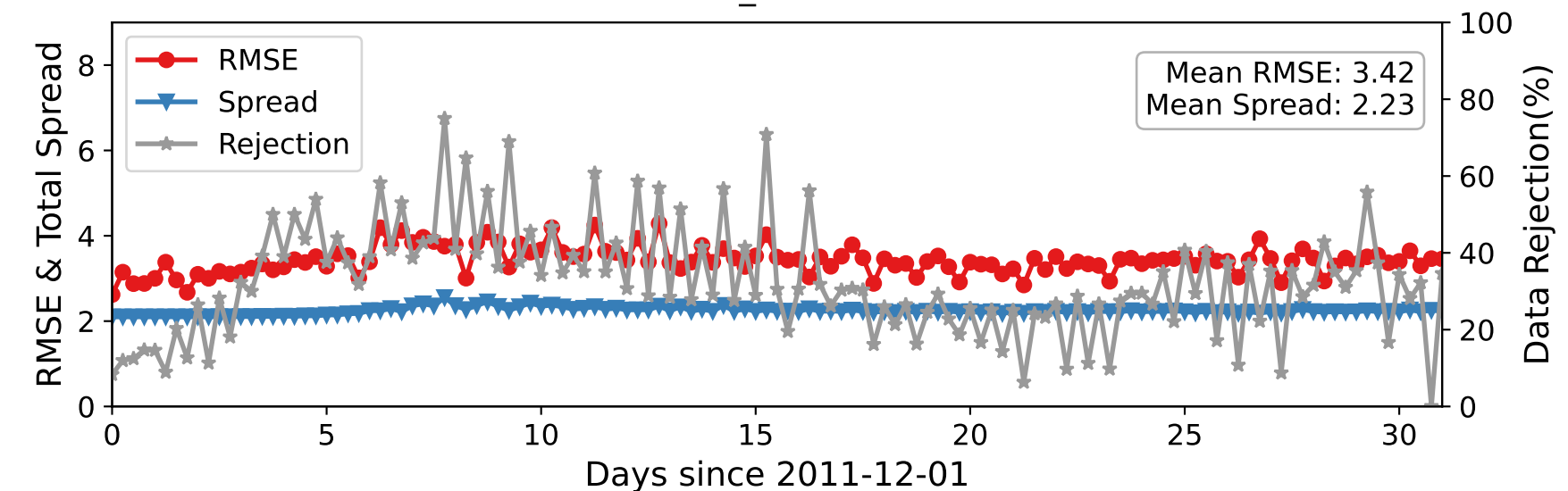
DARTEN40 — U_WIND at 15-35 hPa
