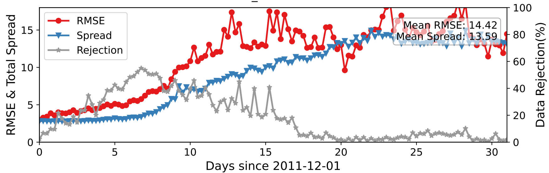
CTRLN10 — U_WIND at 175-225 hPa
