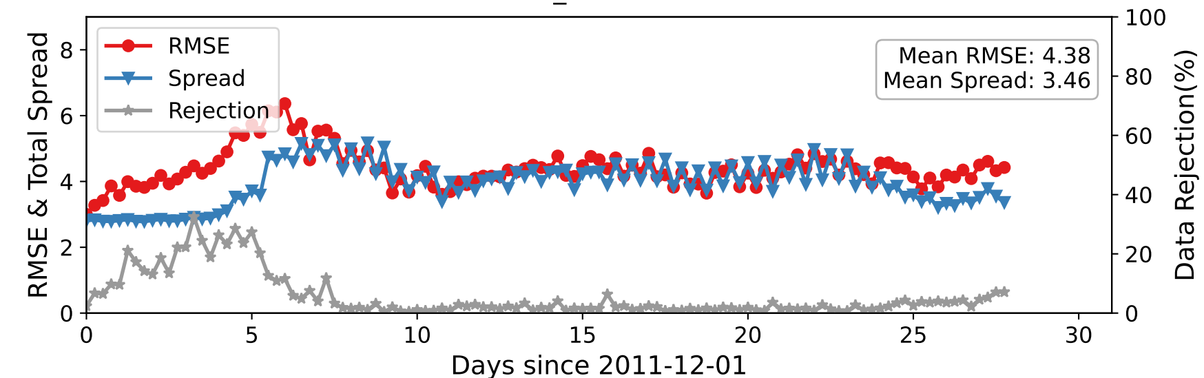
DARTEN10 — U_WIND at 175-225 hPa
