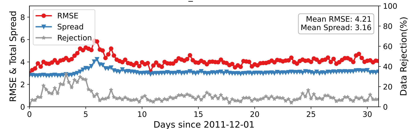
DARTEN40 — U_WIND at 175-225 hPa
