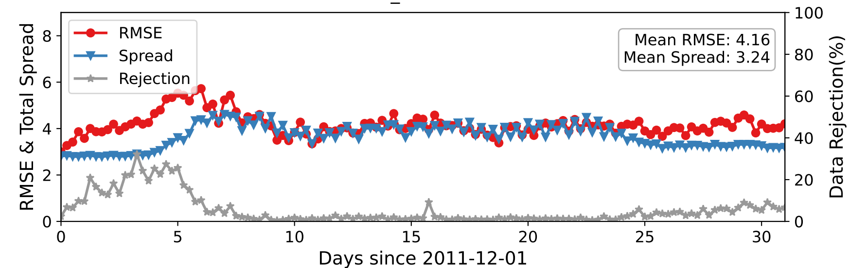
DARTEN20 — U_WIND at 175-225 hPa
