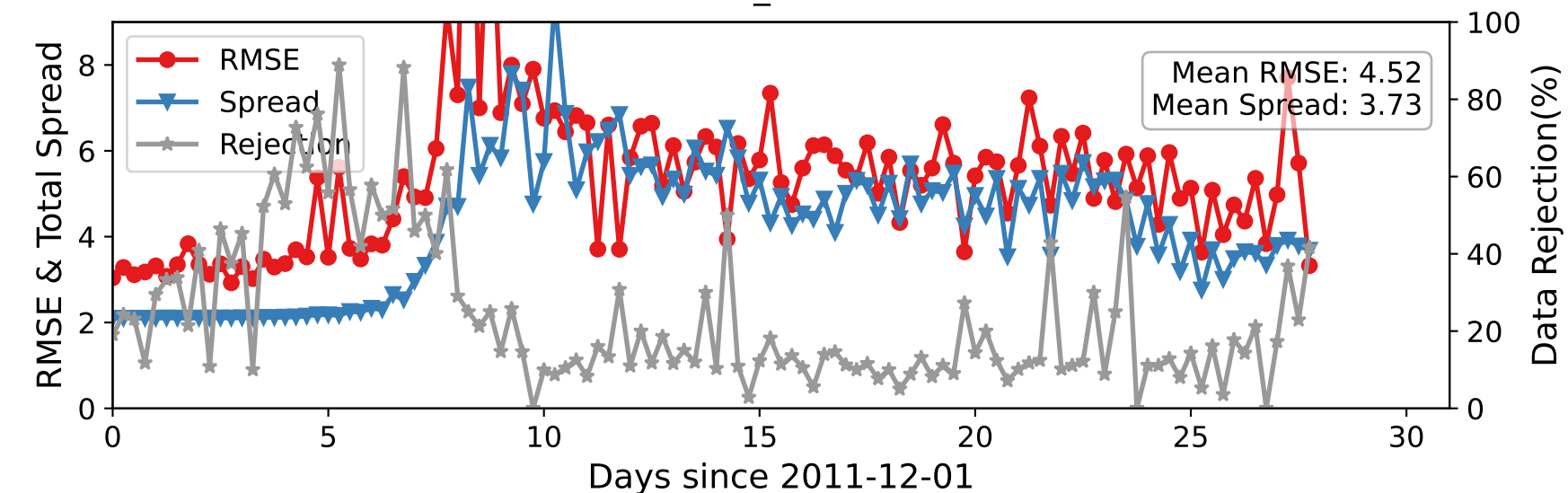
DARTEN10 — U_WIND at 2-15 hPa
