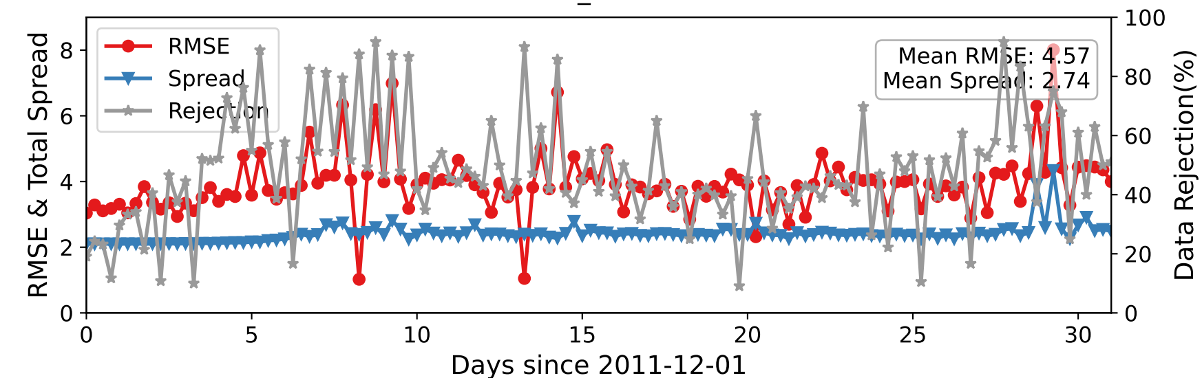
DARTEN40 — U_WIND at 2-15 hPa
