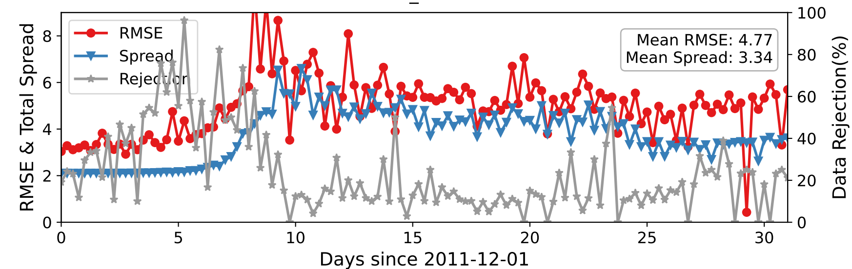
DARTEN20 — U_WIND at 2-15 hPa
