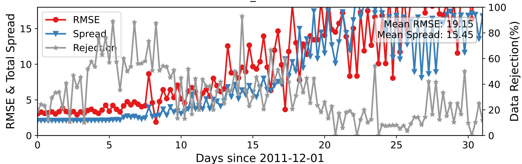
CTRLN10 — U_WIND at 2-15 hPa
