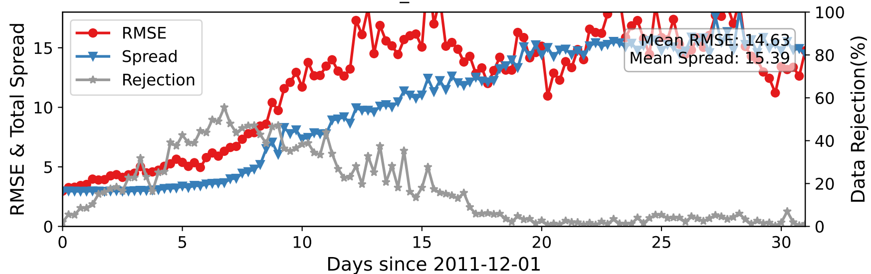
CTRLN10 — U_WIND at 225-275 hPa
