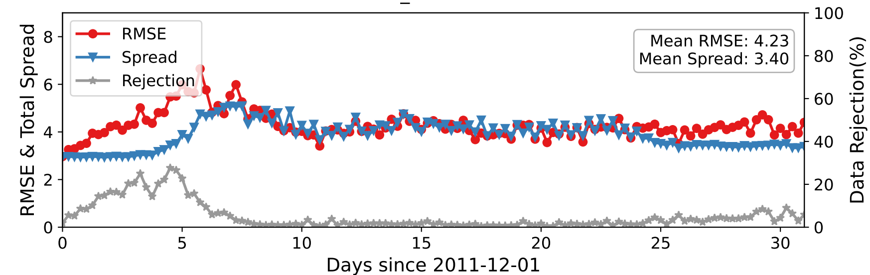
DARTEN20 — U_WIND at 225-275 hPa
