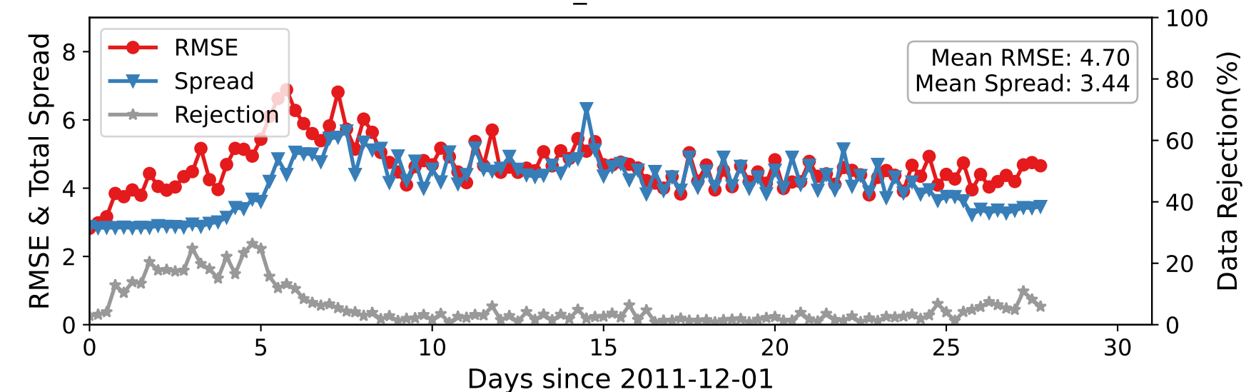
DARTEN10 — U_WIND at 275-350 hPa
