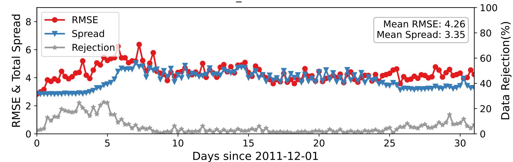
DARTEN20 — U_WIND at 275-350 hPa
