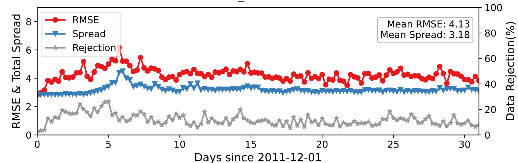
DARTEN40 — U_WIND at 275-350 hPa
