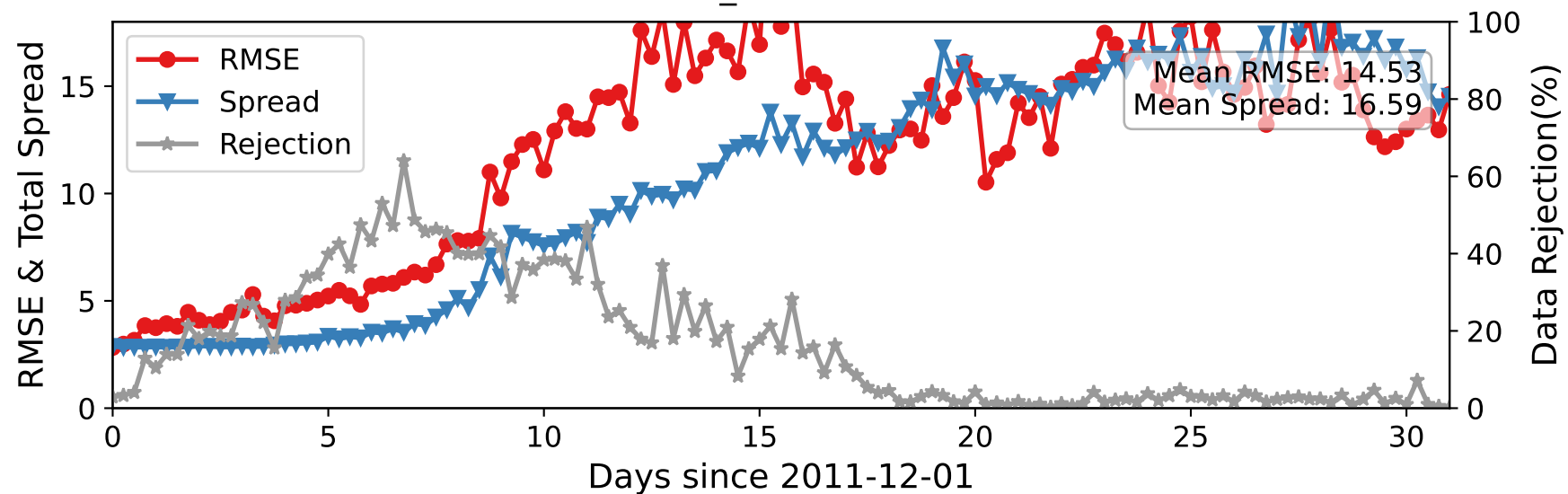
CTRLN10 — U_WIND at 275-350 hPa
