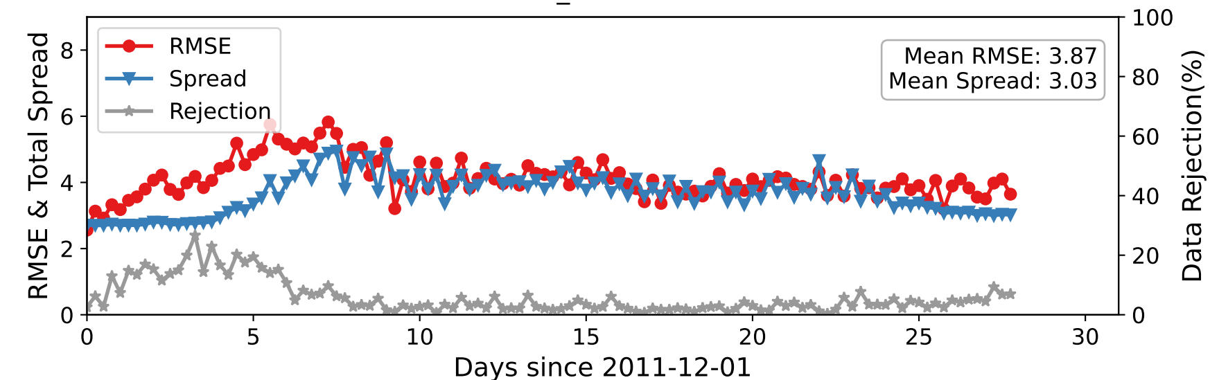
DARTEN10 — U_WIND at 350-450 hPa
