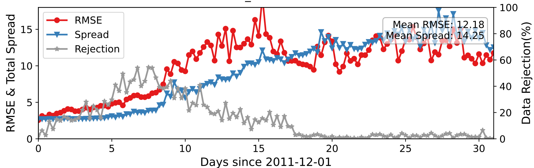
CTRLN10 — U_WIND at 350-450 hPa
