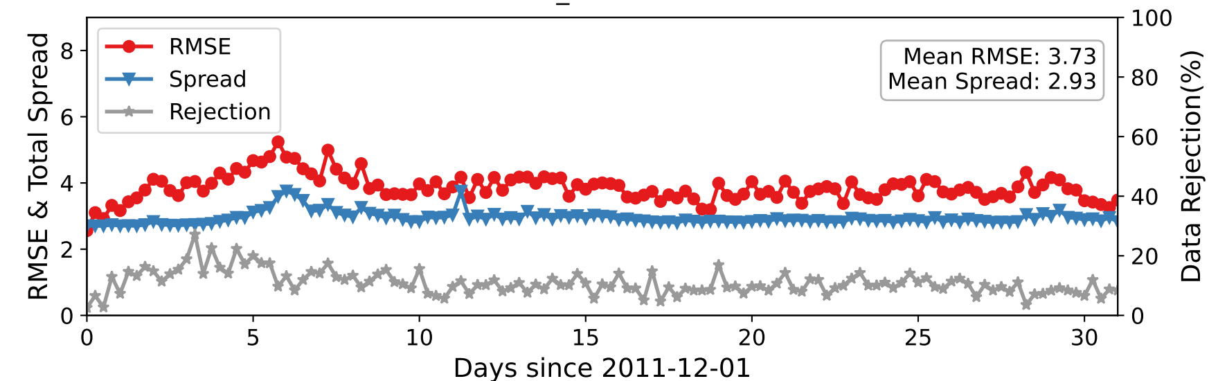
DARTEN40 — U_WIND at 350-450 hPa
