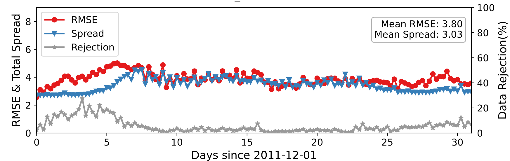
DARTEN20 — U_WIND at 350-450 hPa
