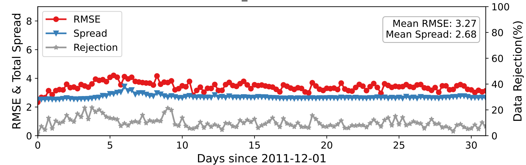
DARTEN40 — U_WIND at 450-600 hPa
