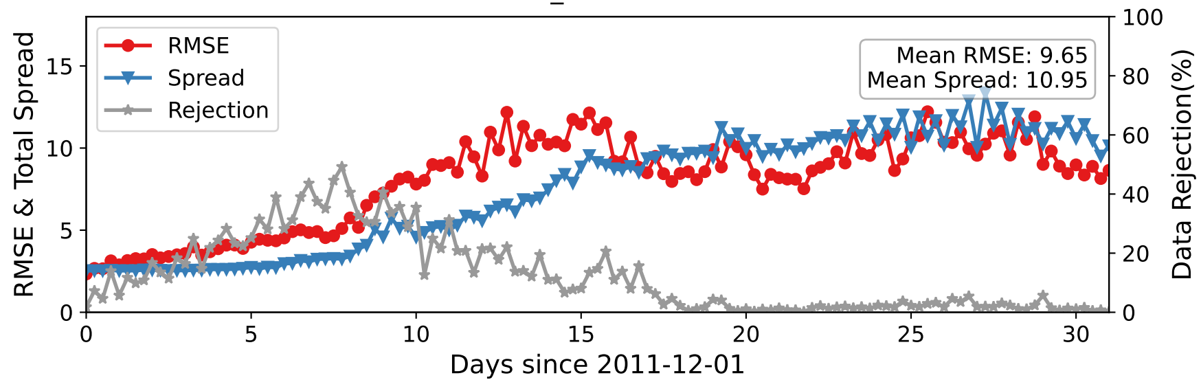
CTRLN10 — U_WIND at 450-600 hPa
