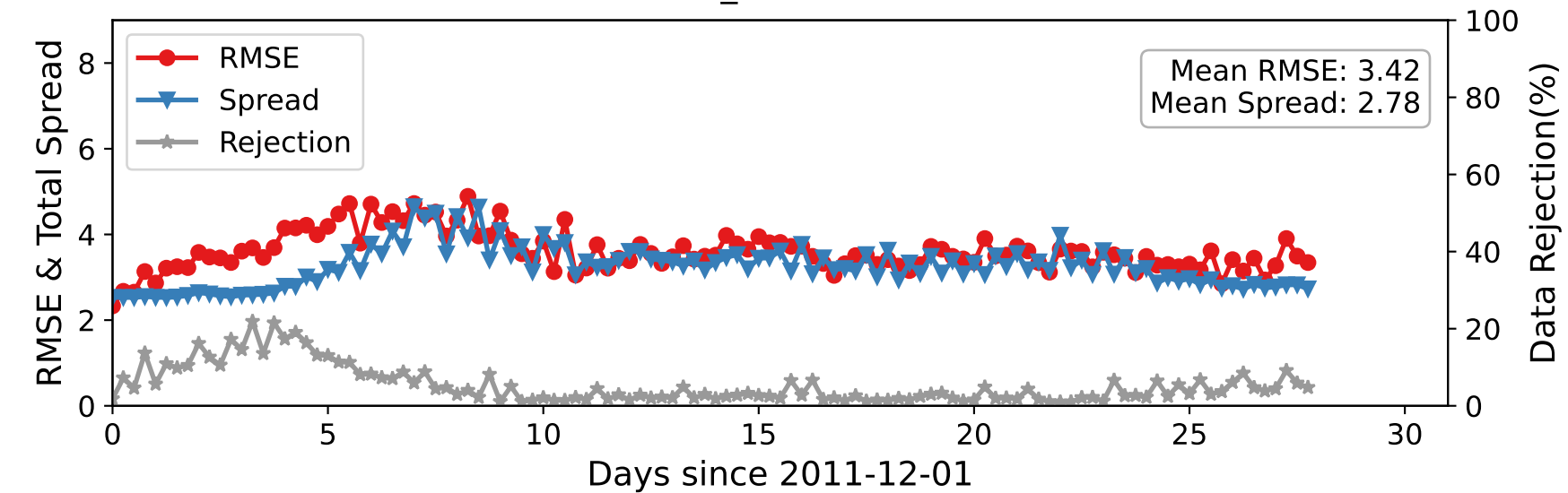
DARTEN10 — U_WIND at 450-600 hPa
