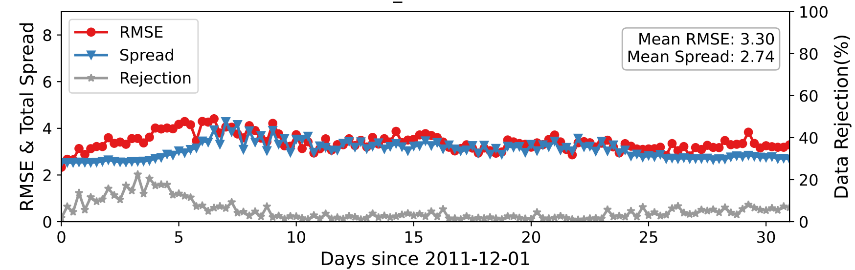
DARTEN20 — U_WIND at 450-600 hPa
