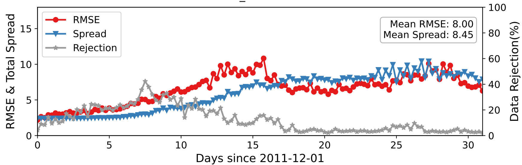
CTRLN10 — U_WIND at 600-775 hPa
