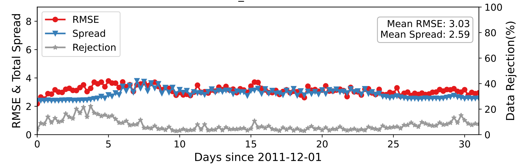
DARTEN20 — U_WIND at 600-775 hPa
