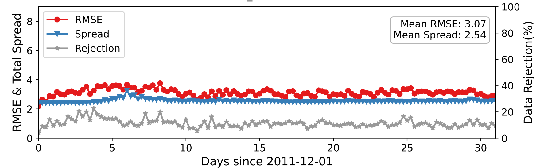
DARTEN40 — U_WIND at 600-775 hPa
