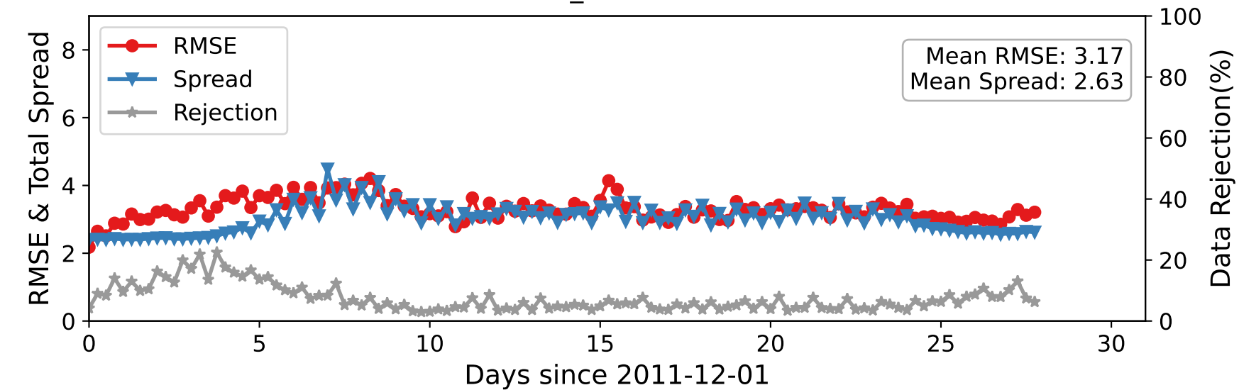
DARTEN10 — U_WIND at 600-775 hPa
