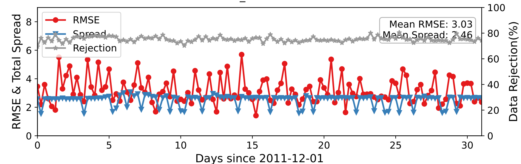
DARTEN40 — U_WIND at 775-887 hPa
