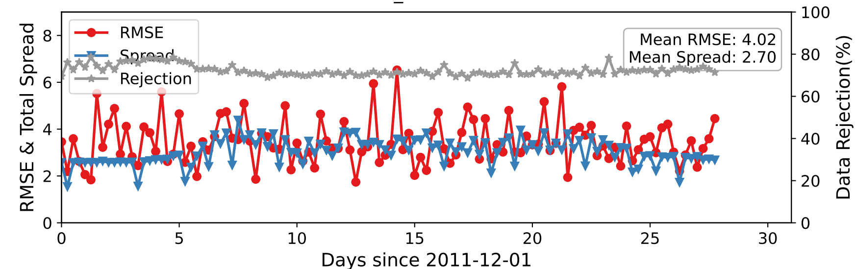
DARTEN10 — U_WIND at 775-887 hPa
