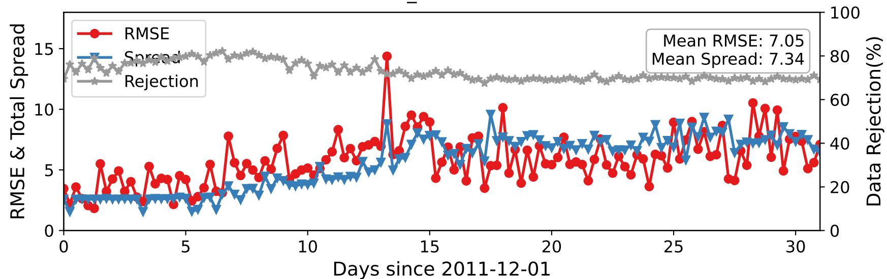
CTRLN10 — U_WIND at 775-887 hPa
