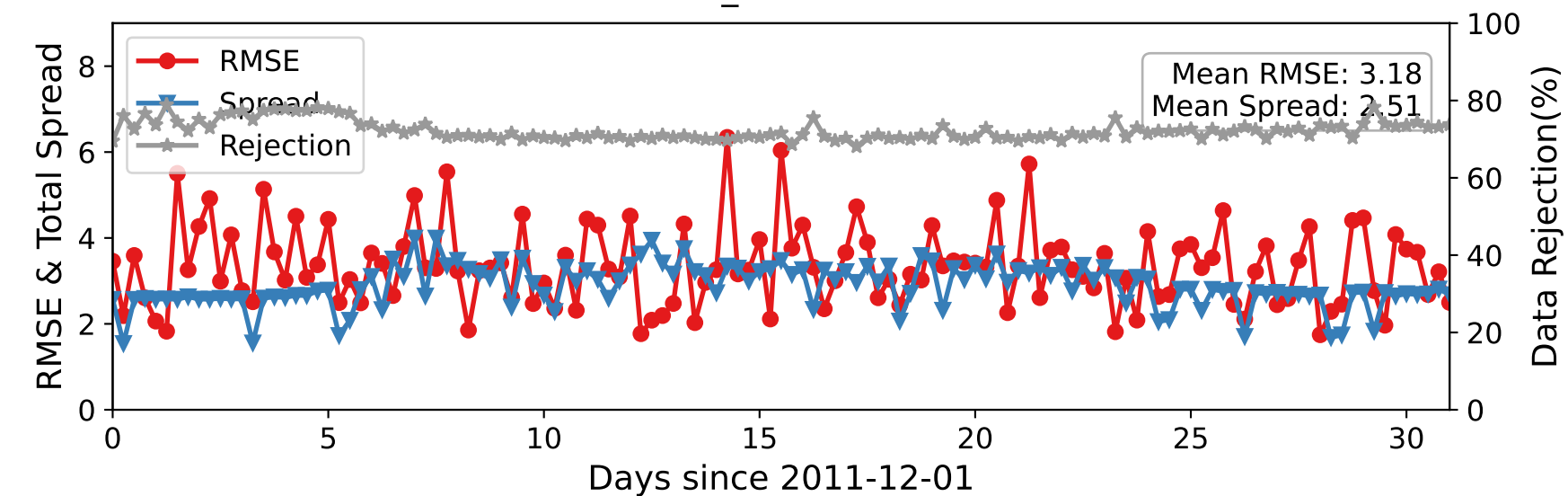
DARTEN20 — U_WIND at 775-887 hPa
