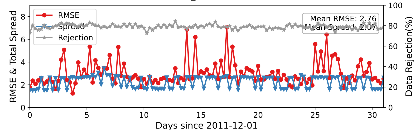
DARTEN40 — U_WIND at 887-962 hPa
