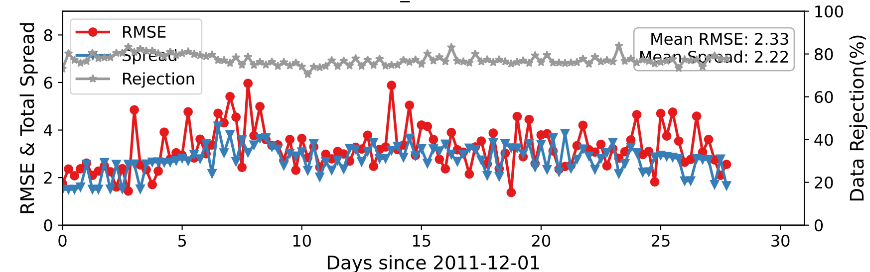
DARTEN10 — U_WIND at 887-962 hPa
