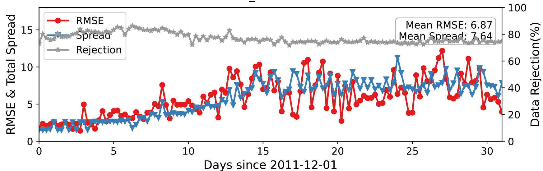
CTRLN10 — U_WIND at 887-962 hPa
