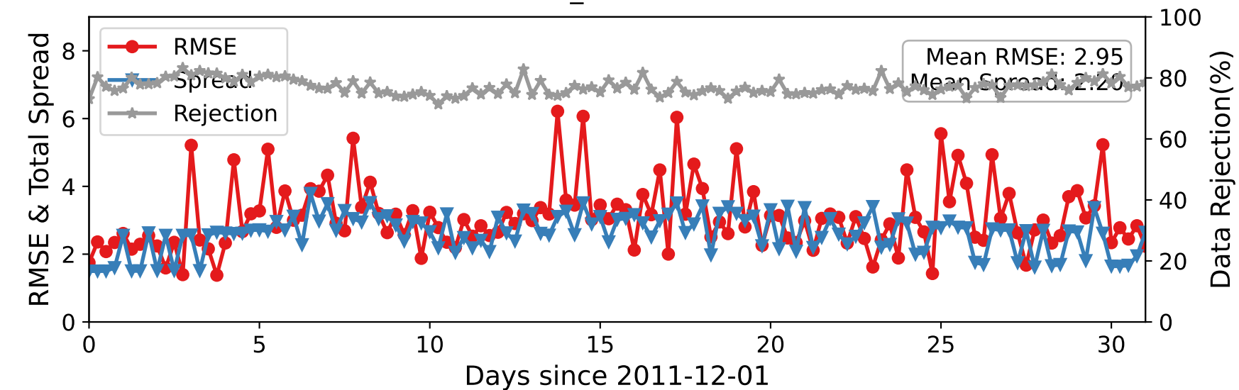
DARTEN20 — U_WIND at 887-962 hPa
