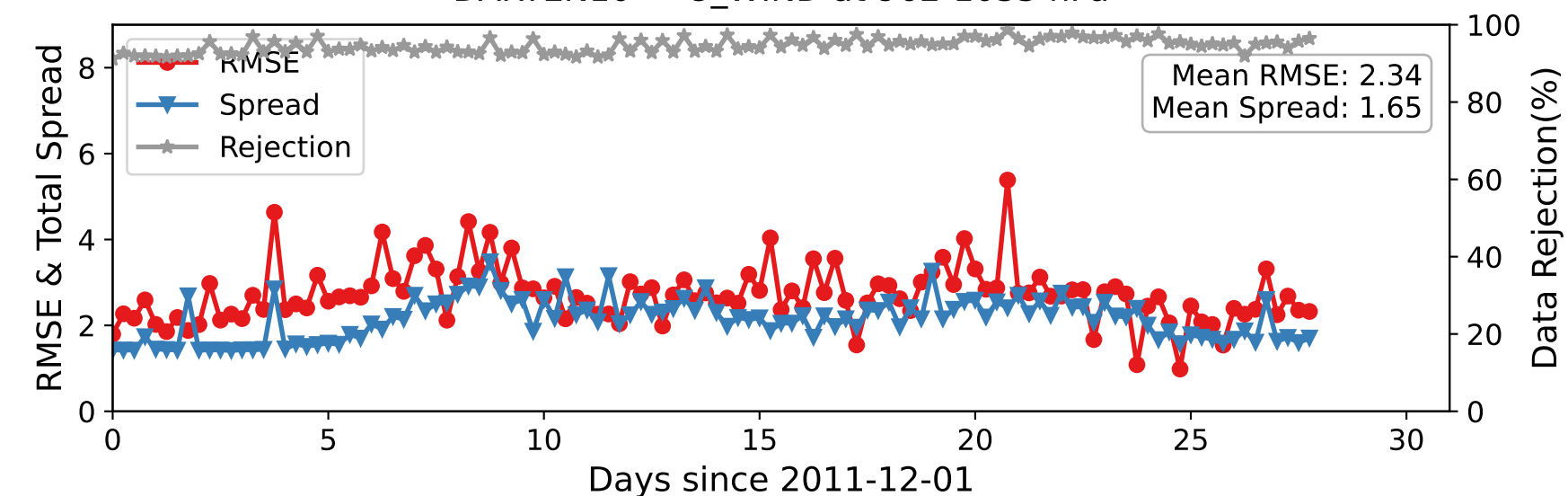
DARTEN10 — U_WIND at 962-1035 hPa
