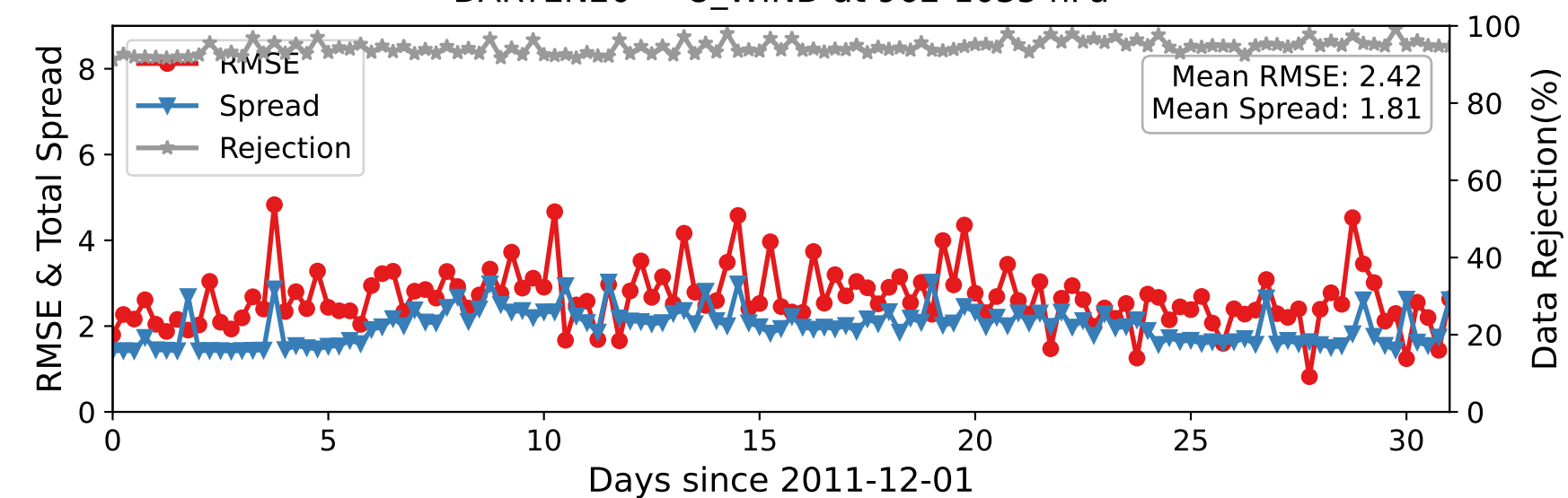
DARTEN20 — U_WIND at 962-1035 hPa
