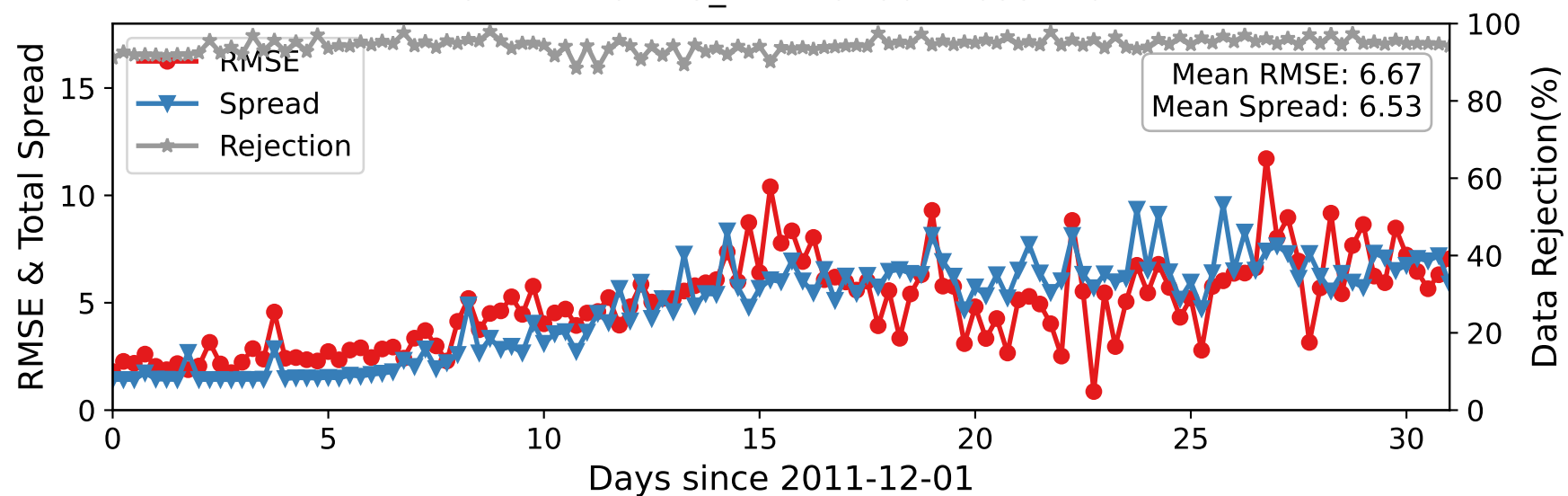
CTRLN10 — U_WIND at 962-1035 hPa
