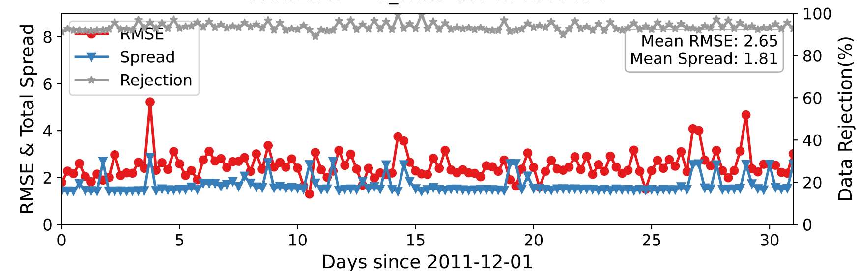
DARTEN40 — U_WIND at 962-1035 hPa
