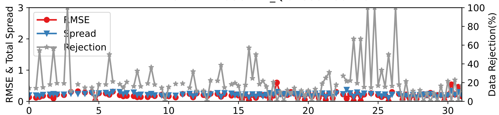
DARTEN20 — RADIOSONDE_Q at 350-450 hPa
