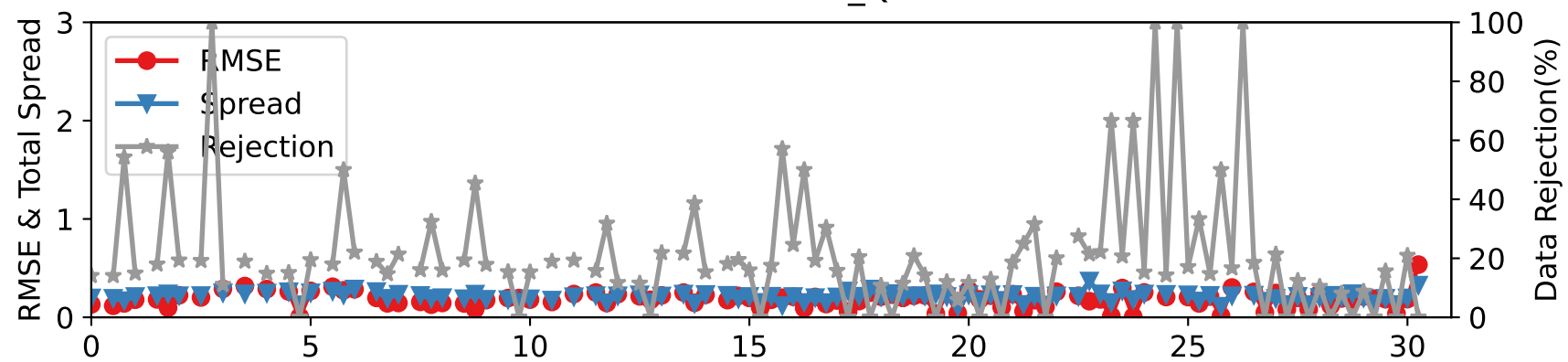
DARTEN40 — RADIOSONDE_Q at 350-450 hPa
