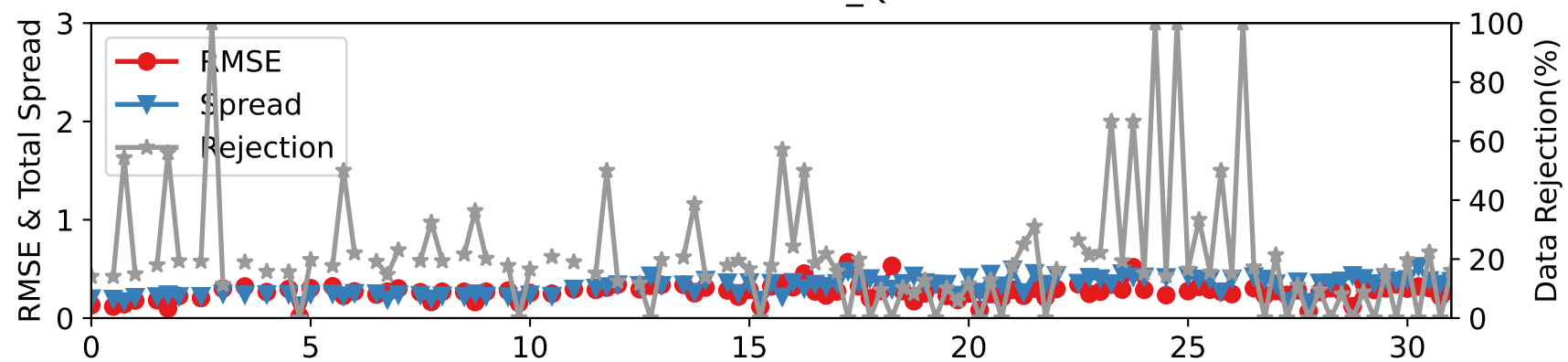
CTRLN10 — RADIOSONDE_Q at 350-450 hPa
