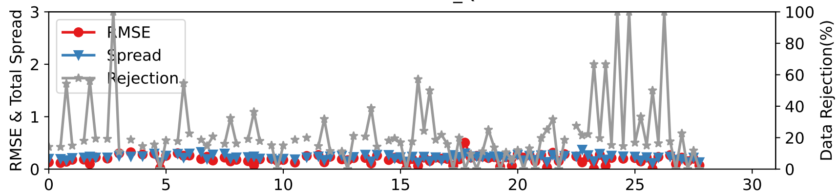
DARTEN10 — RADIOSONDE_Q at 350-450 hPa
