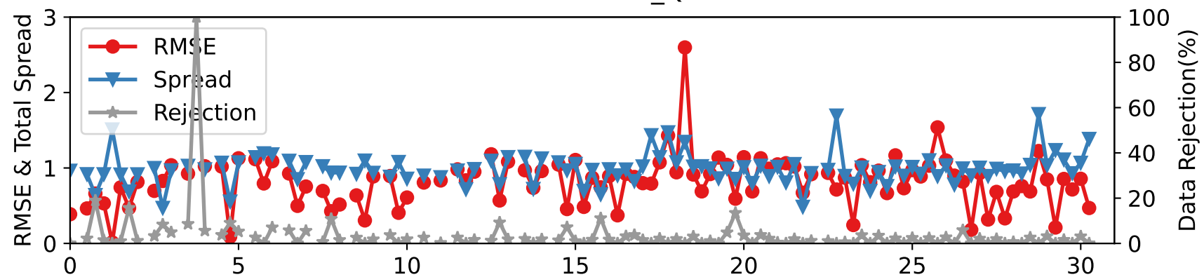
DARTEN40 — RADIOSONDE_Q at 600-775 hPa
