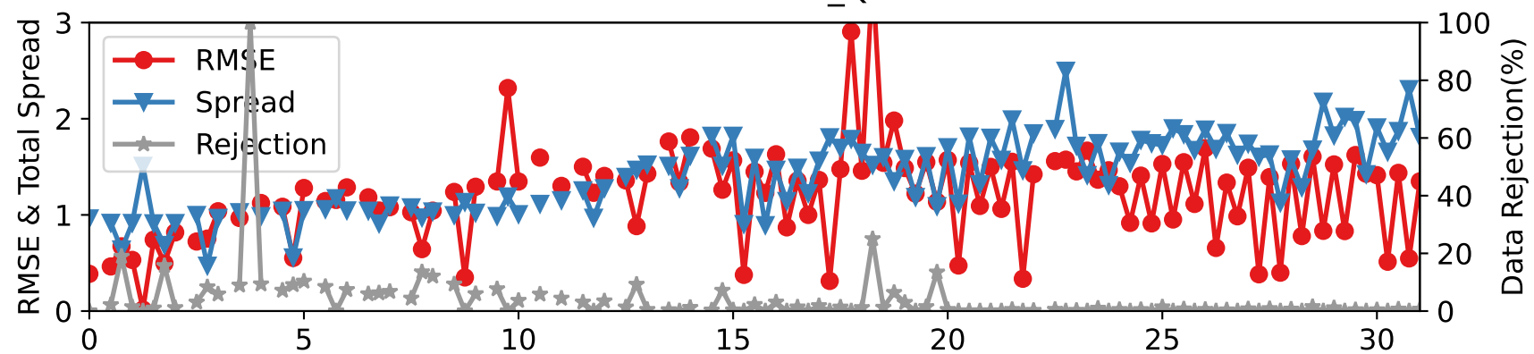
CTRLN10 — RADIOSONDE_Q at 600-775 hPa
