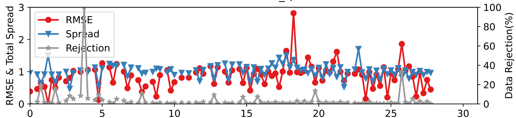
DARTEN10 — RADIOSONDE_Q at 600-775 hPa
