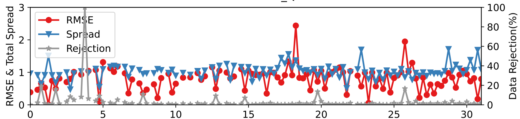
DARTEN20 — RADIOSONDE_Q at 600-775 hPa
