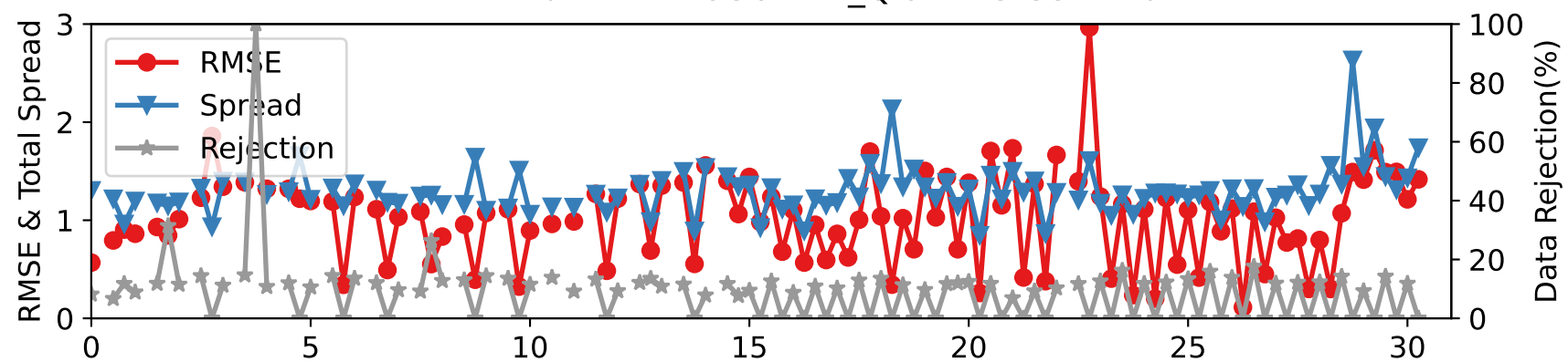
DARTEN40 — RADIOSONDE_Q at 775-887 hPa
