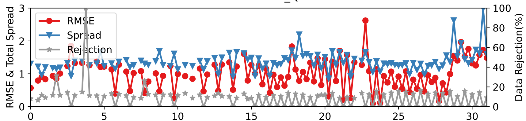
DARTEN20 — RADIOSONDE_Q at 775-887 hPa
