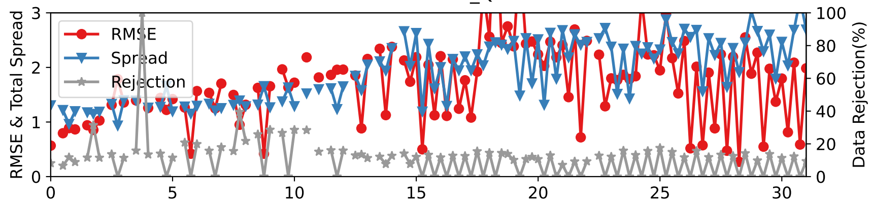
CTRLLEN10 — RADIOSONDE_Q at 775-887 hPa
