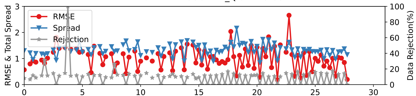
DARTEN10 — RADIOSONDE_Q at 775-887 hPa
