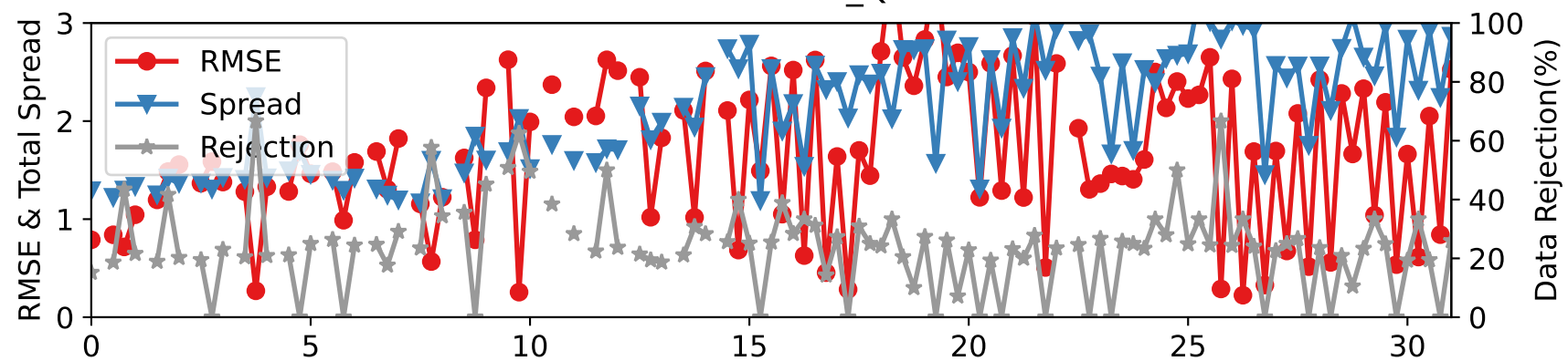
CTRLN10 — RADIOSONDE_Q at 887-962 hPa
