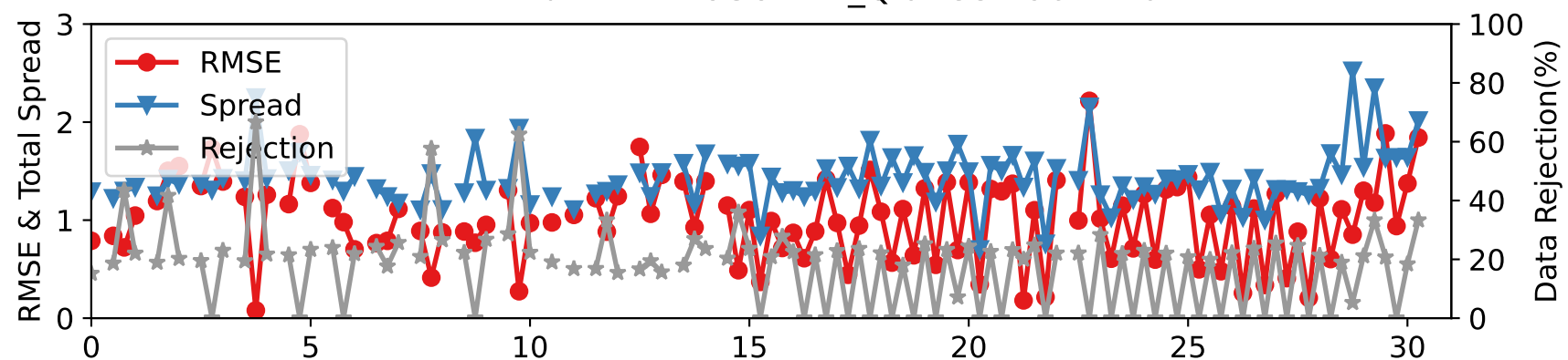
DARTEN40 — RADIOSONDE_Q at 887-962 hPa
