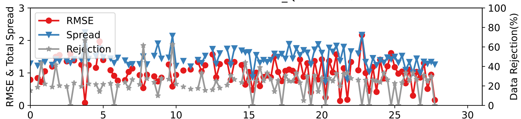
DARTEN10 — RADIOSONDE_Q at 887-962 hPa
