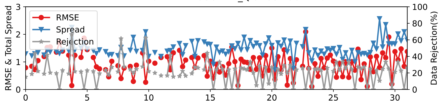
DARTEN20 — RADIOSONDE_Q at 887-962 hPa
