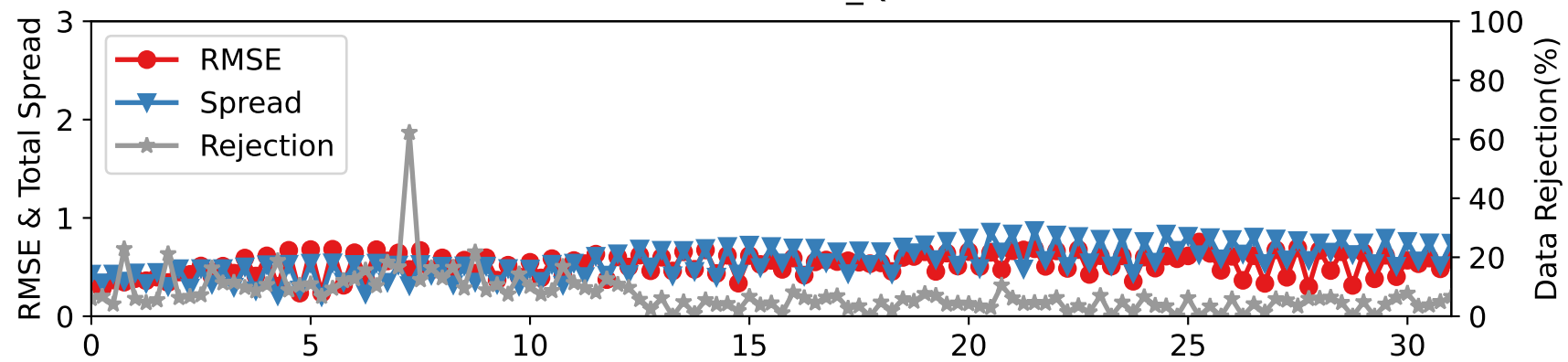
CTRLN10 — RADIOSONDE_Q at 450-600 hPa
