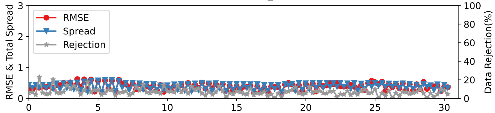
DARTEN40 — RADIOSONDE_Q at 450-600 hPa
