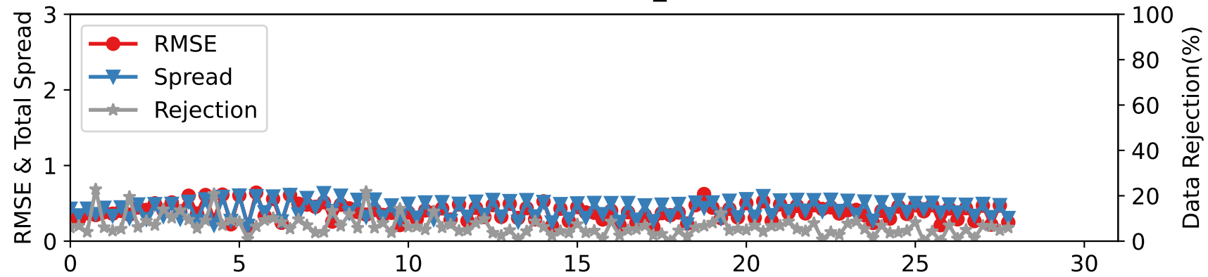
DARTEN10 — RADIOSONDE_Q at 450-600 hPa
