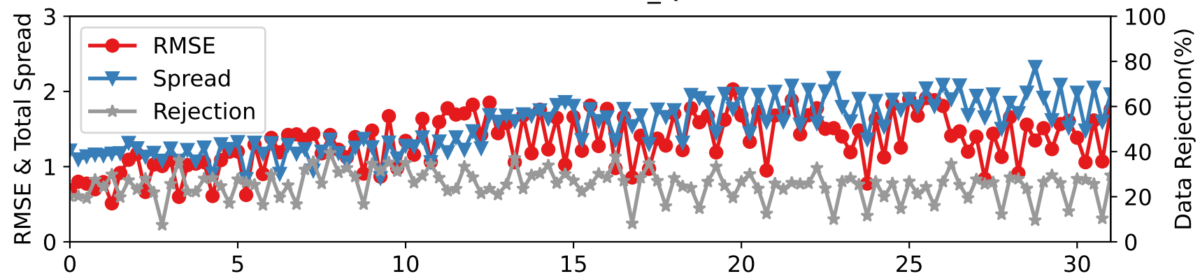
CTRLLEN10 — RADIOSONDE_Q at 887-962 hPa
