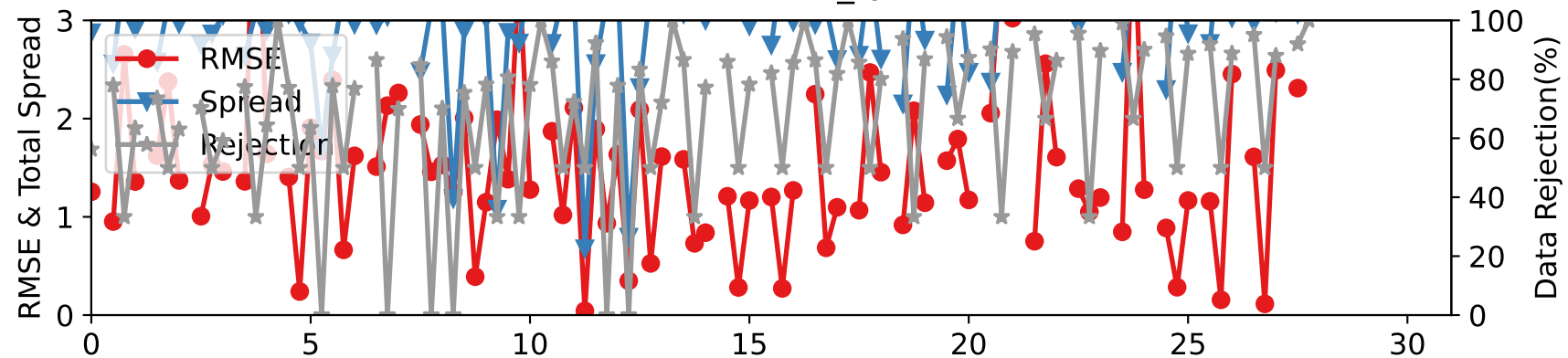
DARTEN10 — RADIOSONDE_Q at 962-1035 hPa
