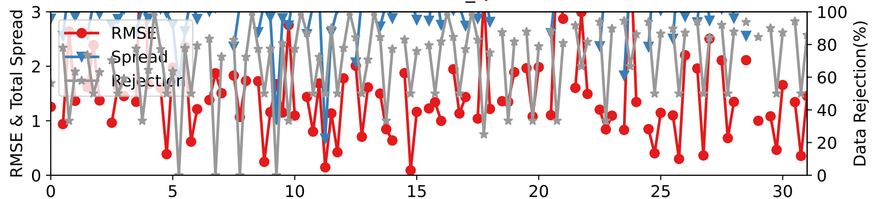
DARTEN20 — RADIOSONDE_Q at 962-1035 hPa
