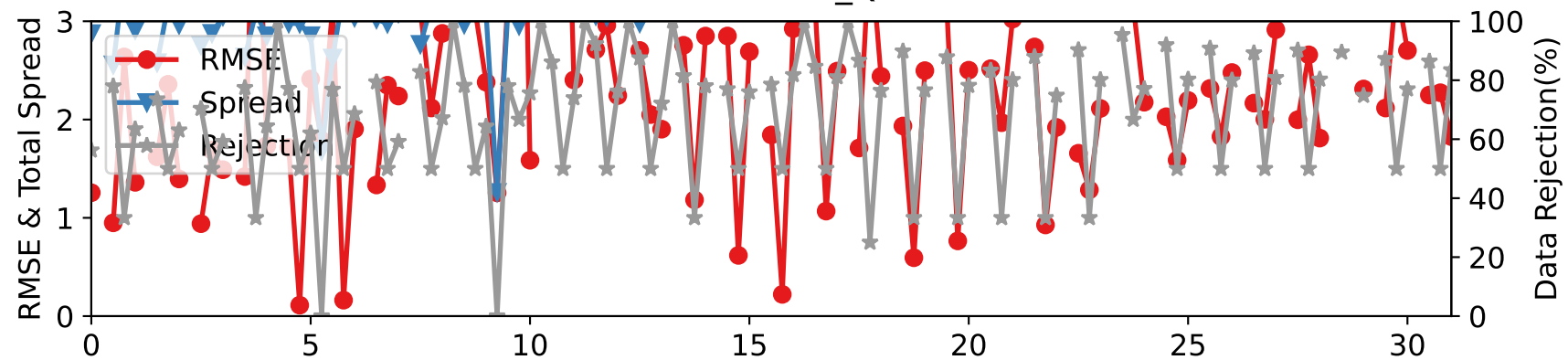
CTRLN10 — RADIOSONDE_Q at 962-1035 hPa
