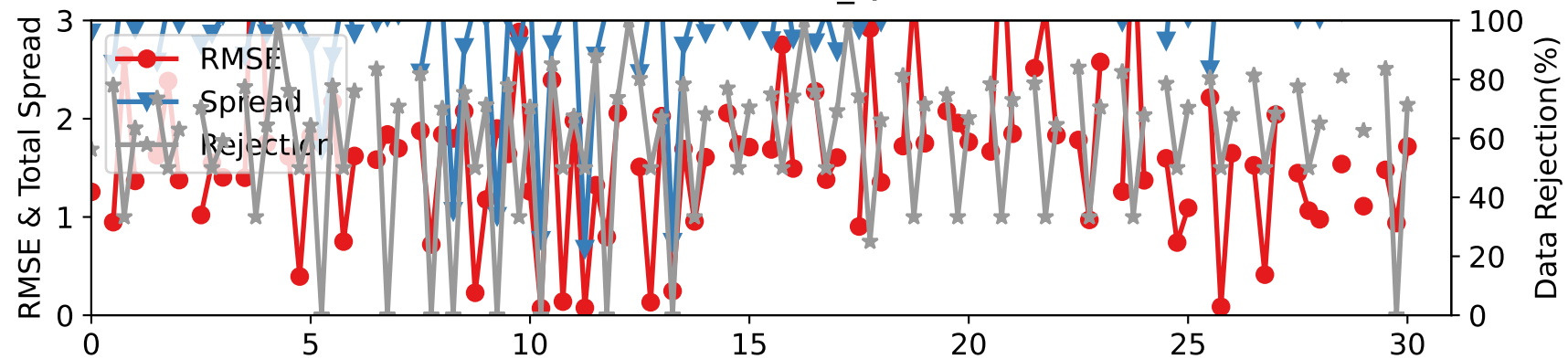
DARTEN40 — RADIOSONDE_Q at 962-1035 hPa
