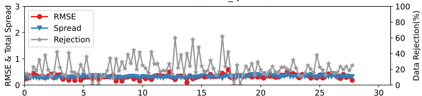
DARTEN10 — RADIOSONDE_Q at 275-350 hPa
