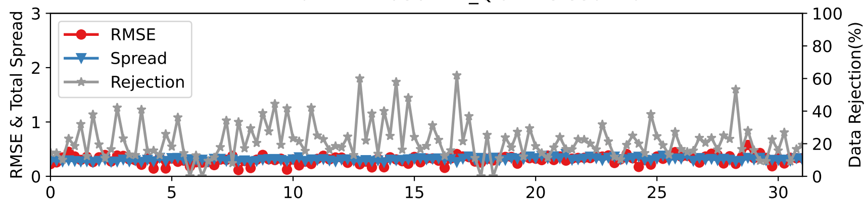
DARTEN20 — RADIOSONDE_Q at 275-350 hPa
