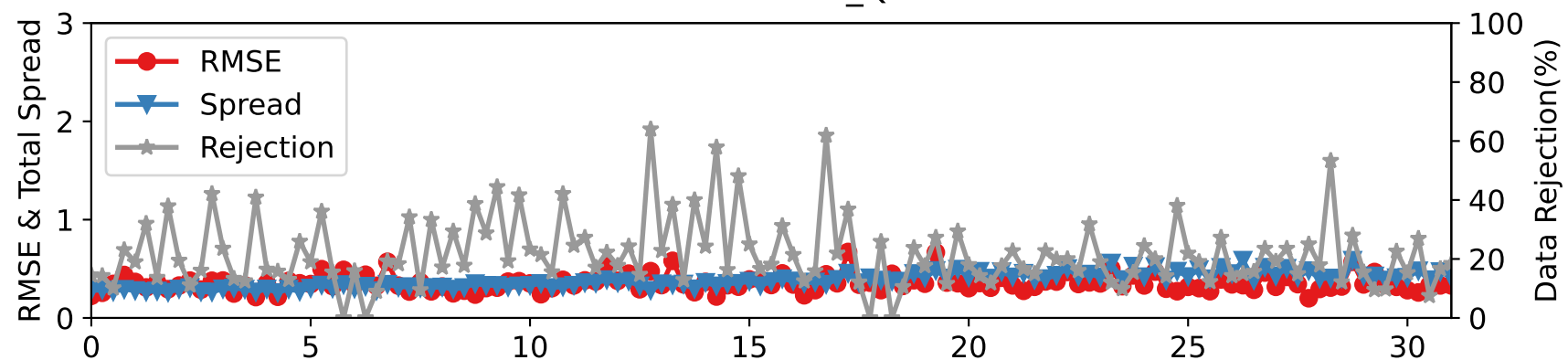
CTRLN10 — RADIOSONDE_Q at 275-350 hPa
