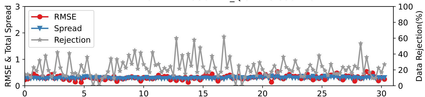
DARTEN40 — RADIOSONDE_Q at 275-350 hPa
