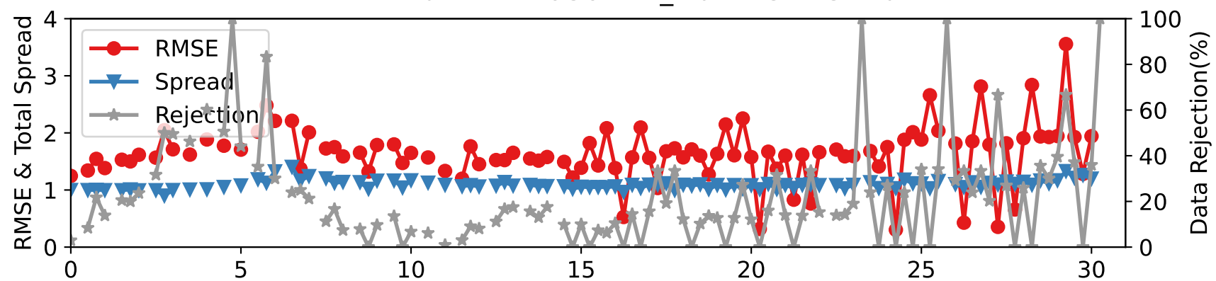
DARTEN40 — RADIOSONDE_T at 125-175 hPa
