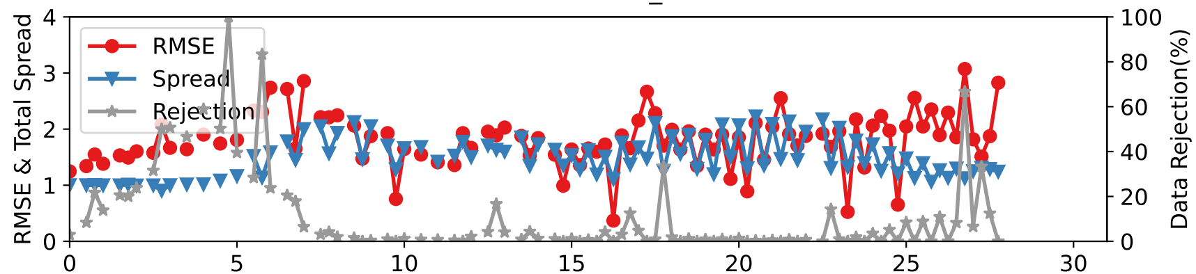
DARTEN10 — RADIOSONDE_T at 125-175 hPa
