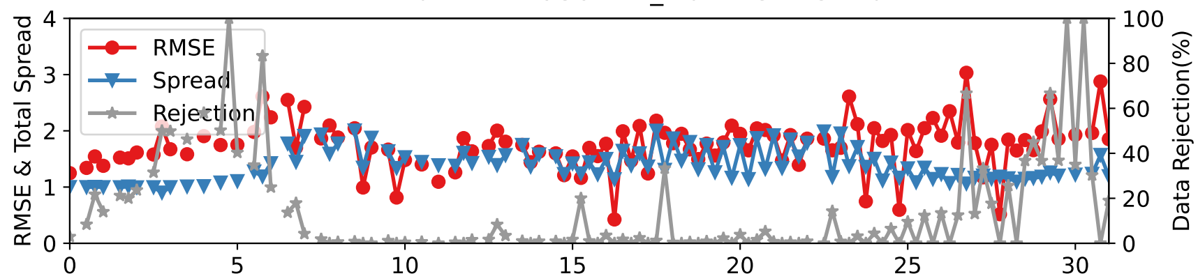
DARTEN20 — RADIOSONDE_T at 125-175 hPa
