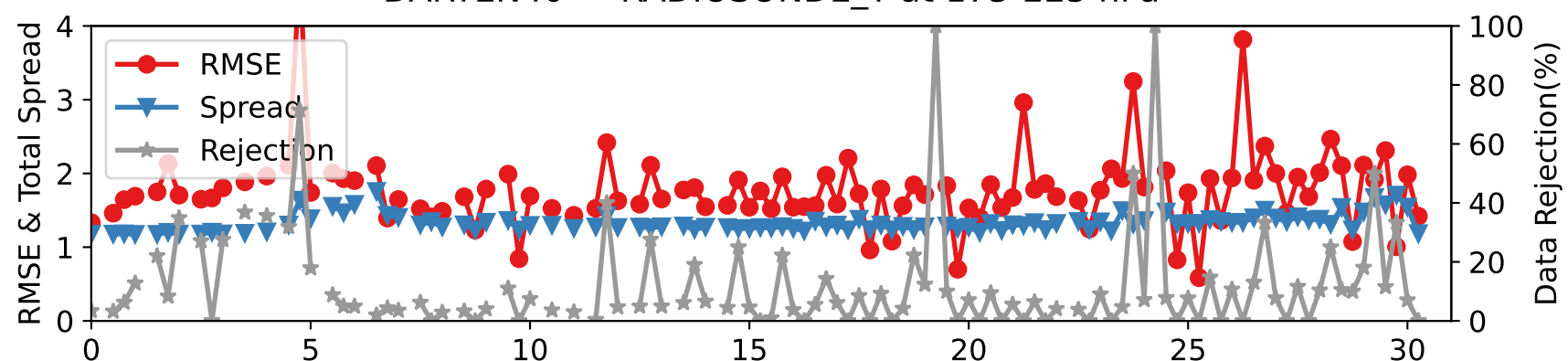
DARTEN40 — RADIOSONDE_T at 175-225 hPa
