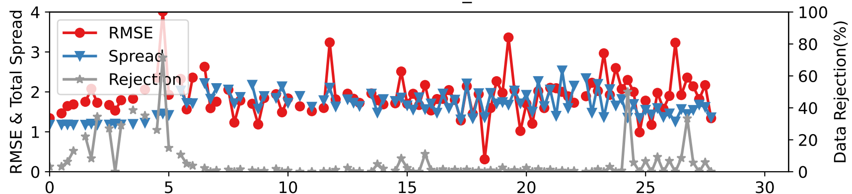
DARTEN10 — RADIOSONDE_T at 175-225 hPa
