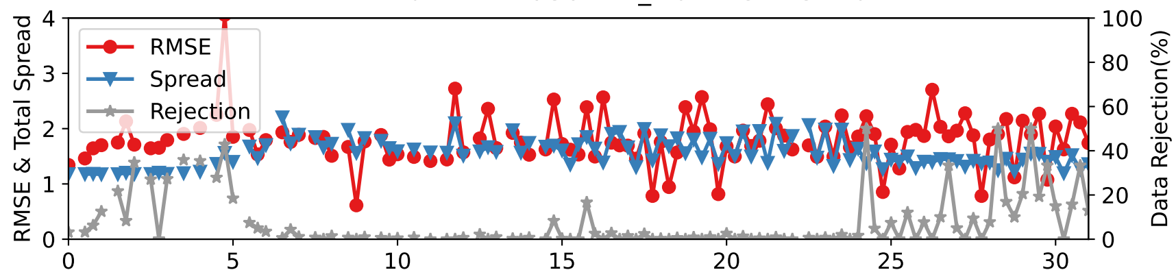
DARTEN20 — RADIOSONDE_T at 175-225 hPa
