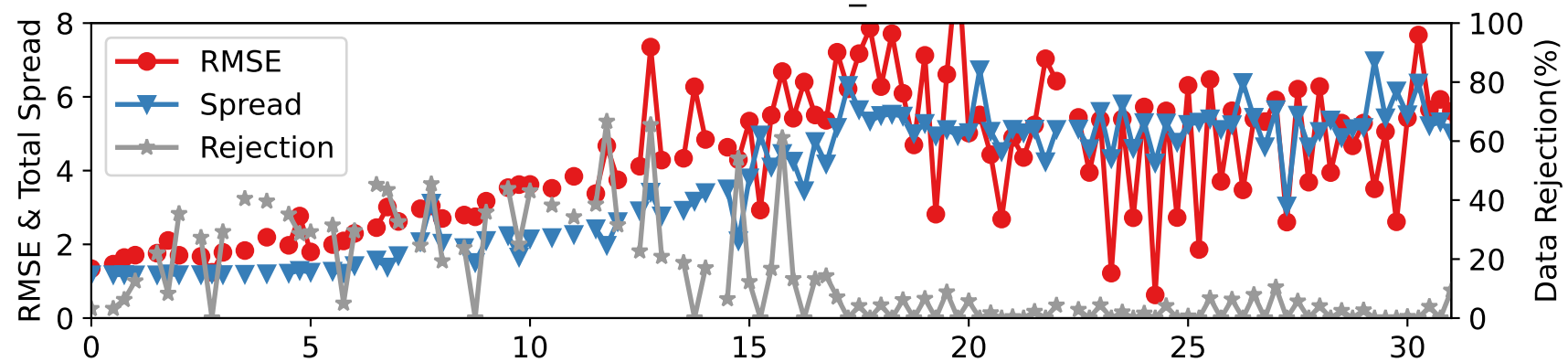
CTRLN10 — RADIOSONDE_T at 175-225 hPa
