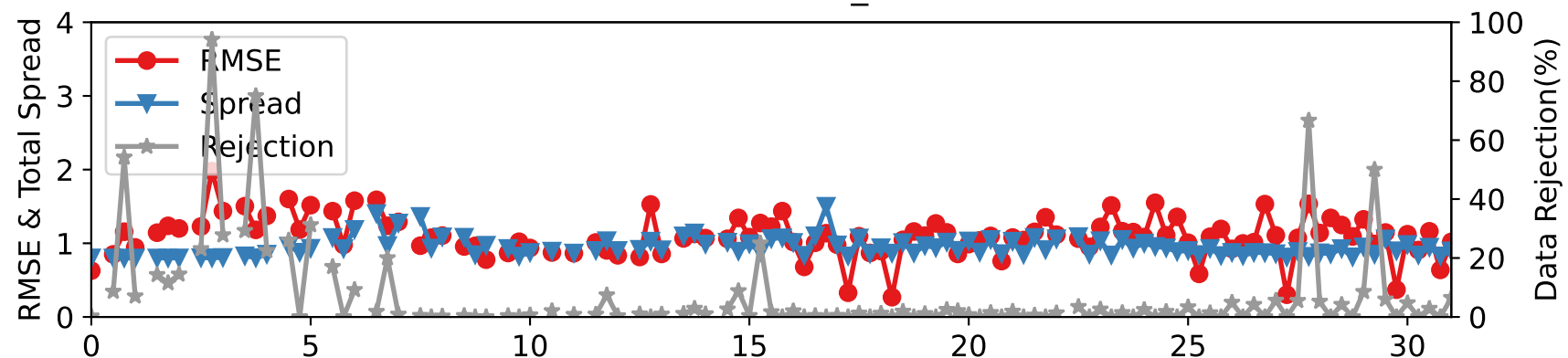
DARTEN20 — RADIOSONDE_T at 450-600 hPa
