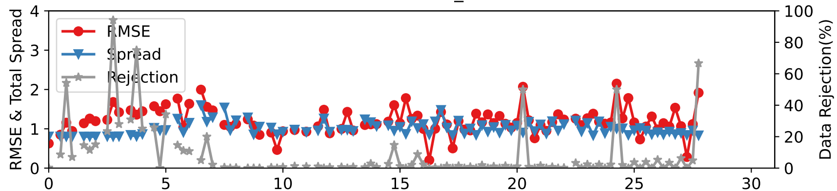
DARTEN10 — RADIOSONDE_T at 450-600 hPa
