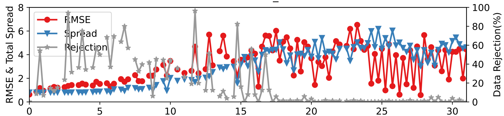
CTRLN10 — RADIOSONDE_T at 450-600 hPa
