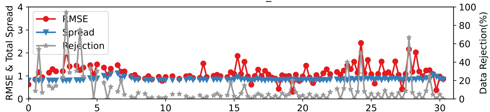
DARTEN40 — RADIOSONDE_T at 450-600 hPa
