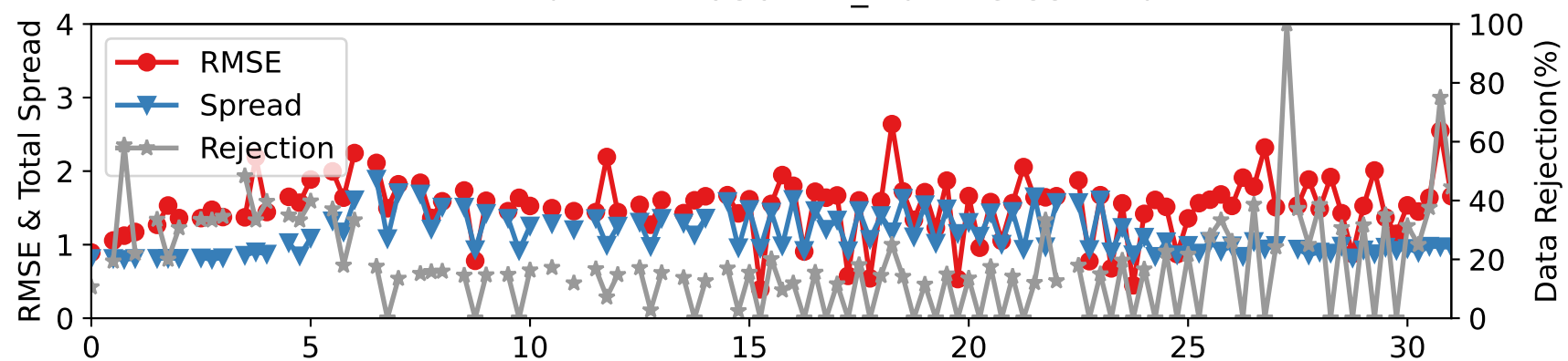
DARTEN20 — RADIOSONDE_T at 775-887 hPa
