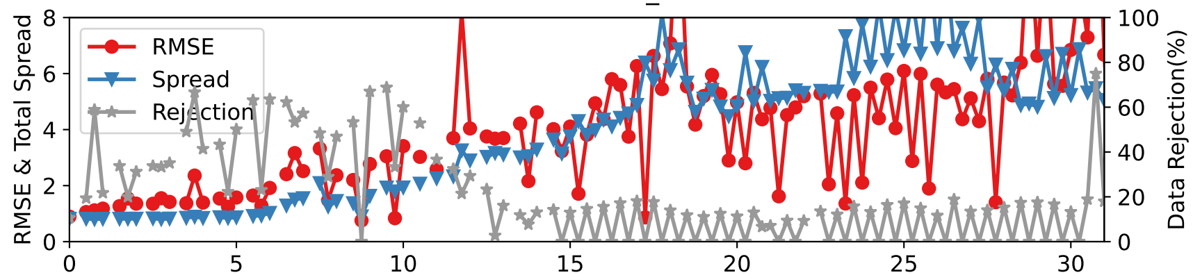
CTRLN10 — RADIOSONDE_T at 775-887 hPa
