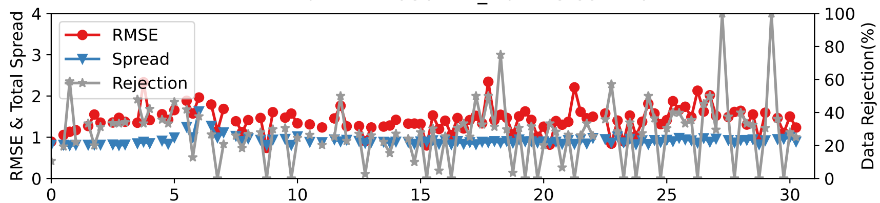
DARTEN40 — RADIOSONDE_T at 775-887 hPa
