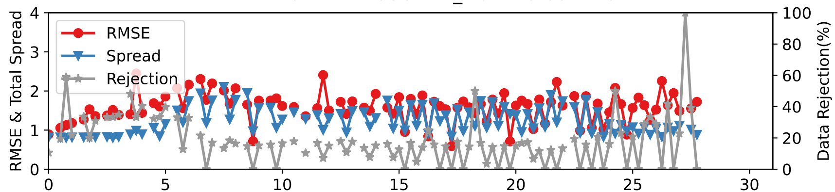
DARTEN10 — RADIOSONDE_T at 775-887 hPa
