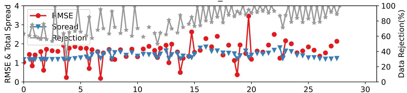
DARTEN10 — RADIOSONDE_T at 962-1035 hPa
