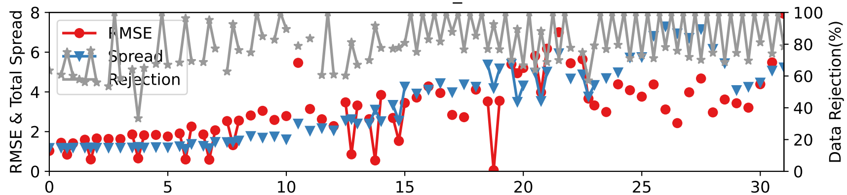
CTRLN10 — RADIOSONDE_T at 962-1035 hPa
