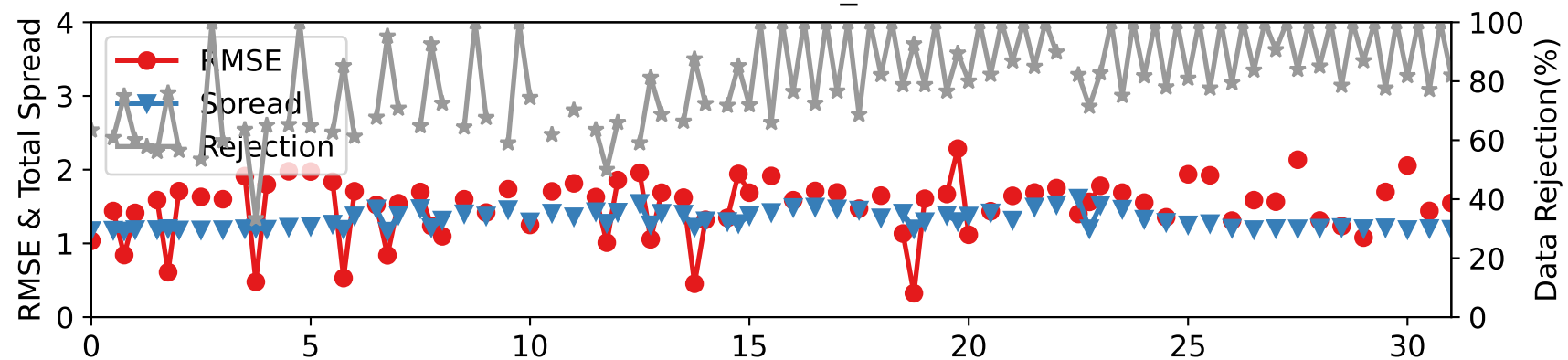
DARTEN20 — RADIOSONDE_T at 962-1035 hPa
