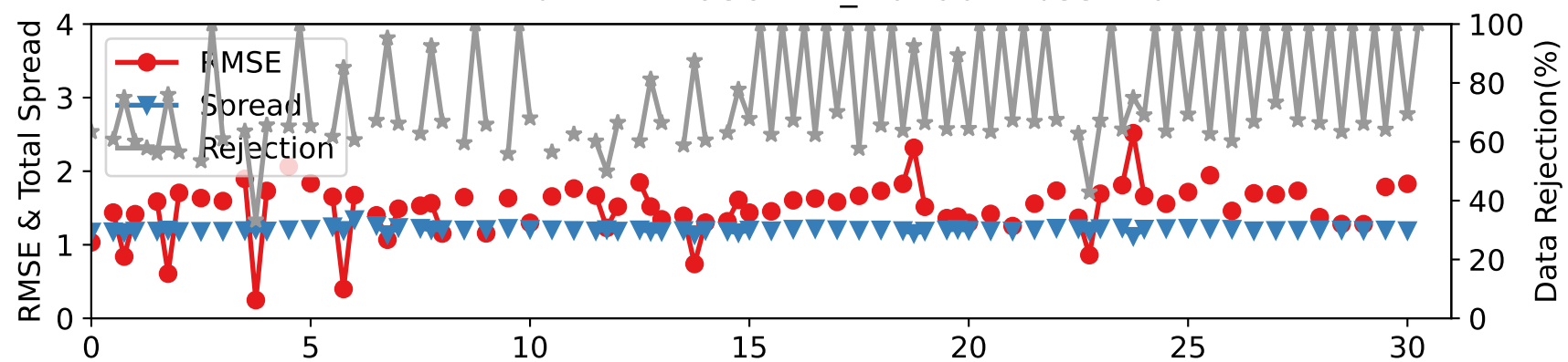
DARTEN40 — RADIOSONDE_T at 962-1035 hPa
