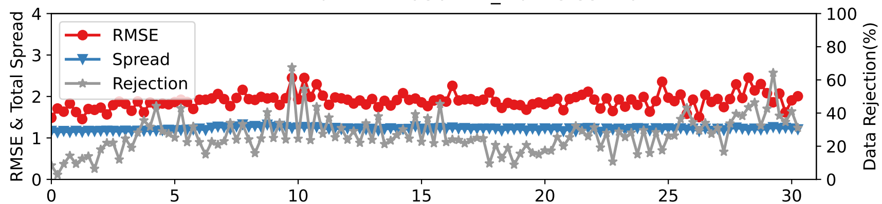
DARTEN40 — RADIOSONDE_T at 15-35 hPa
