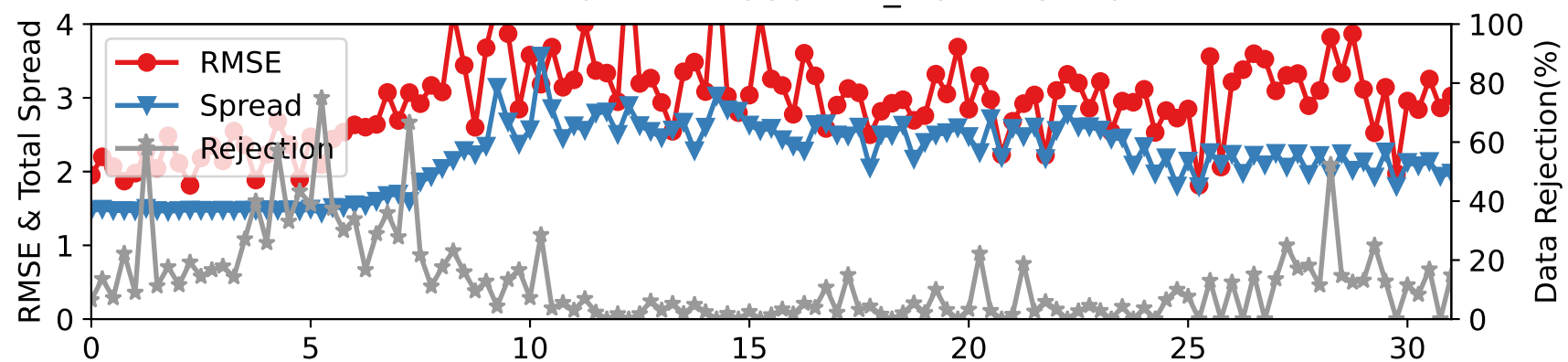
DARTEN20 — RADIOSONDE_T at 2-15 hPa
