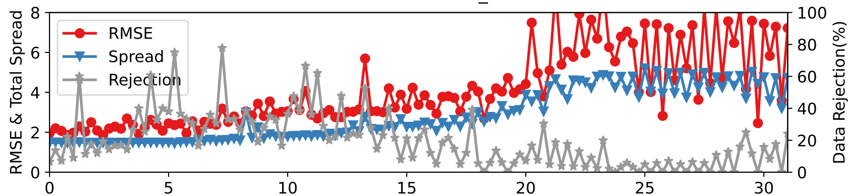
CTRLN10 — RADIOSONDE_T at 2-15 hPa
