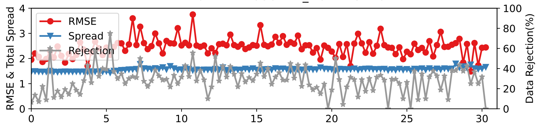
DARTEN40 — RADIOSONDE_T at 2-15 hPa
