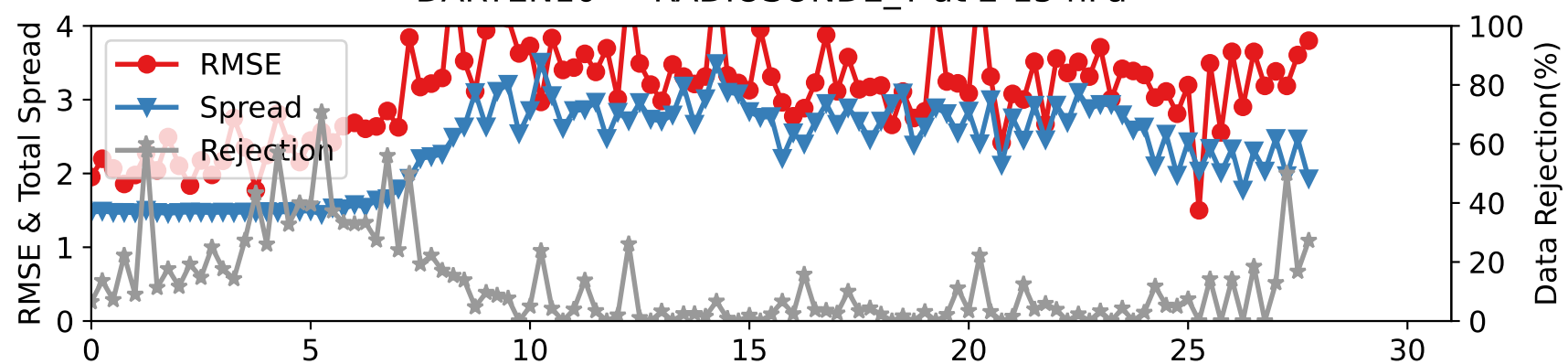
DARTEN10 — RADIOSONDE_T at 2-15 hPa
