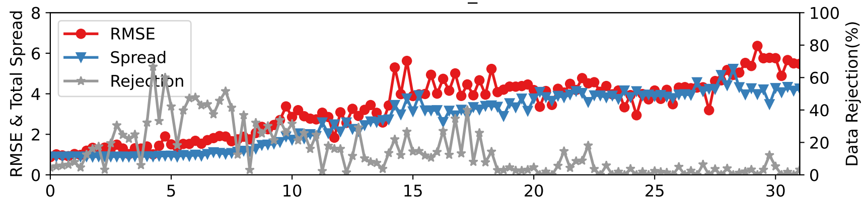
CTRLN10 — RADIOSONDE_T at 275-350 hPa
