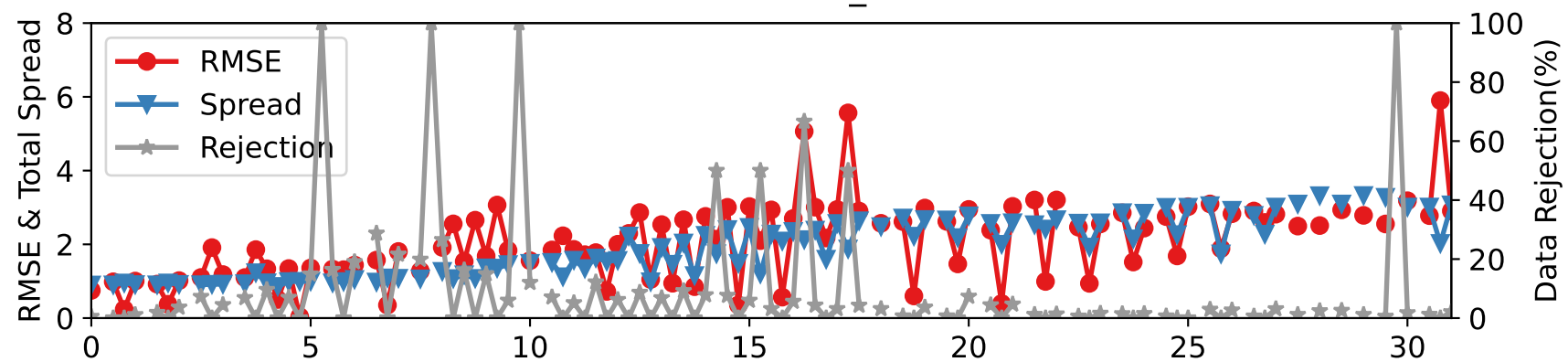
CTRLLEN10 — RADIOSONDE_T at 275-350 hPa
