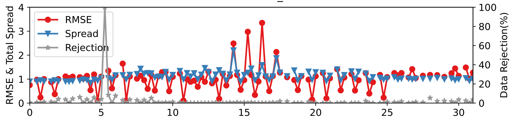
DARTEN20 — RADIOSONDE_T at 275-350 hPa
