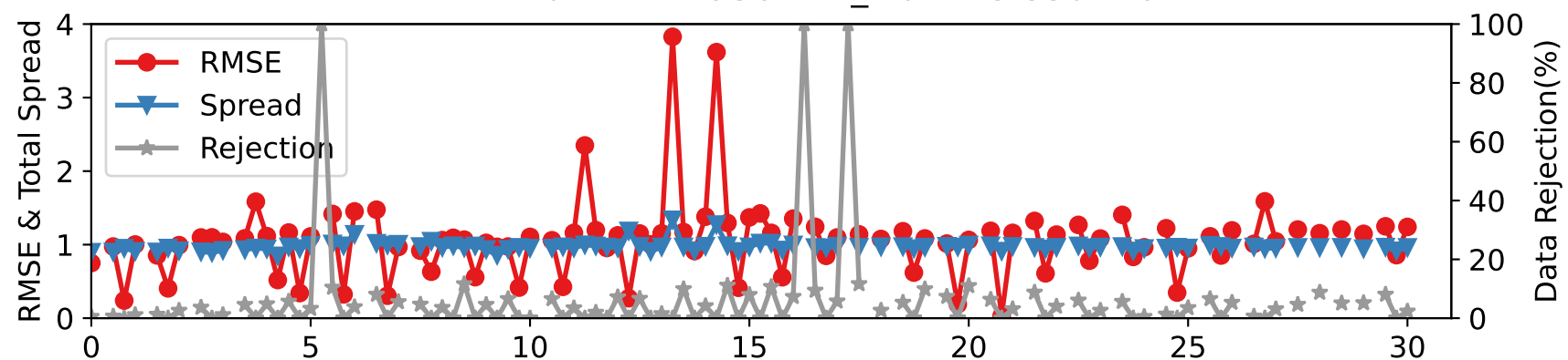
DARTEN40 — RADIOSONDE_T at 275-350 hPa
