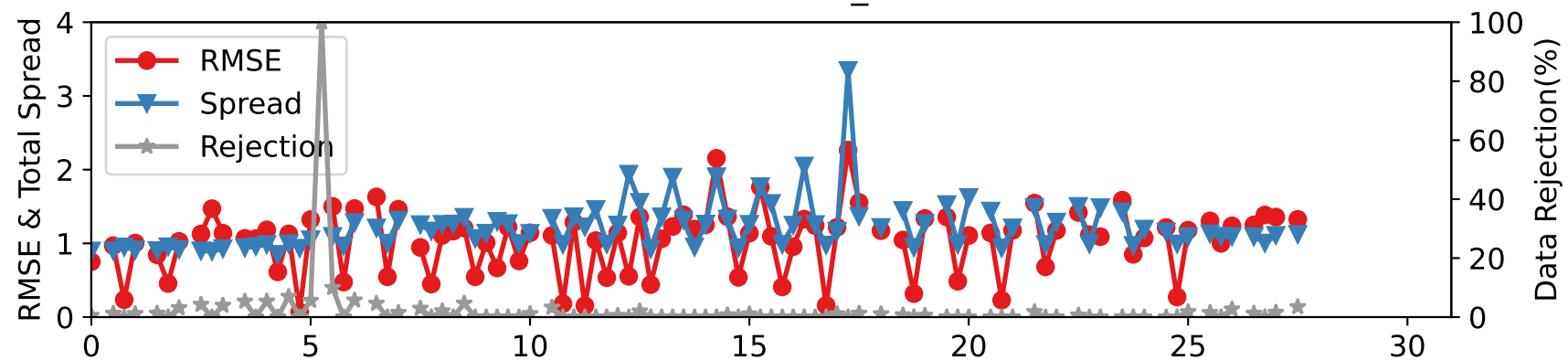
DARTEN10 — RADIOSONDE_T at 275-350 hPa
