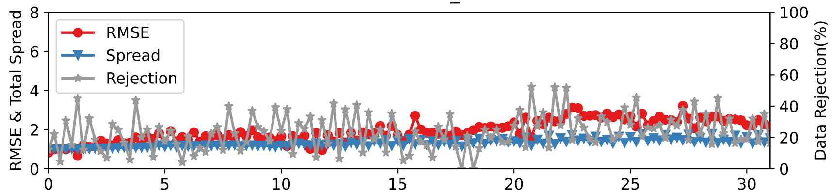
CTRLN10 — RADIOSONDE_T at 125-175 hPa
