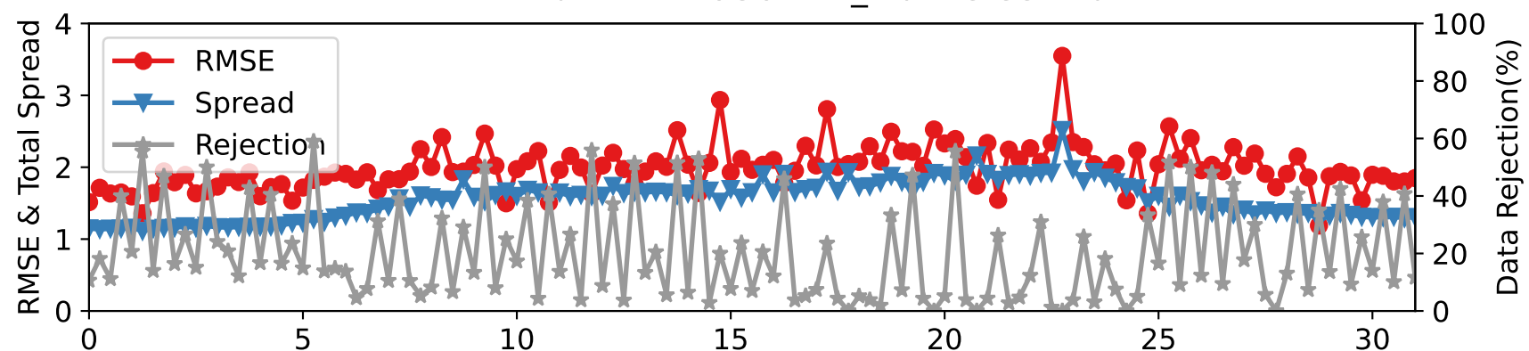
DARTEN20 — RADIOSONDE_T at 15-35 hPa
