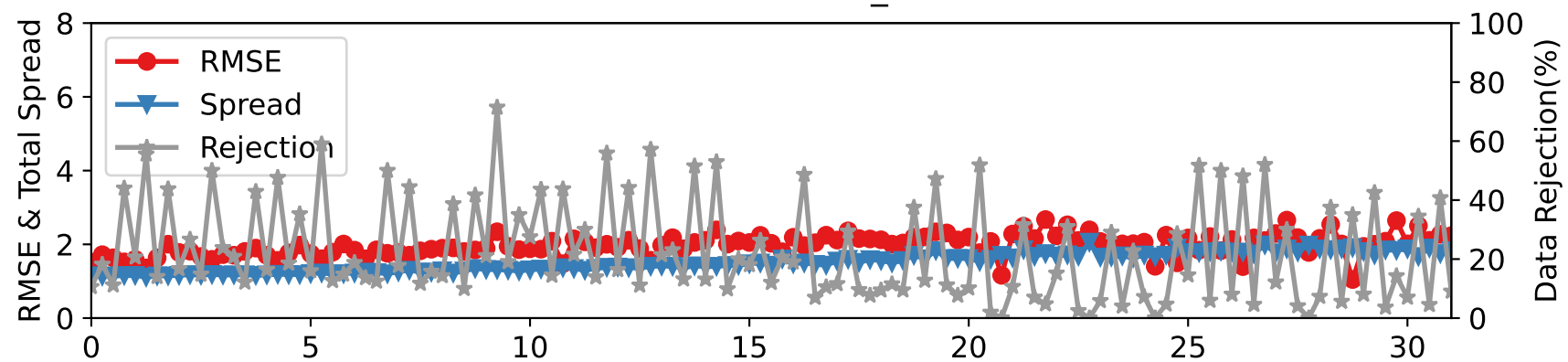
CTRLN10 — RADIOSONDE_T at 15-35 hPa
