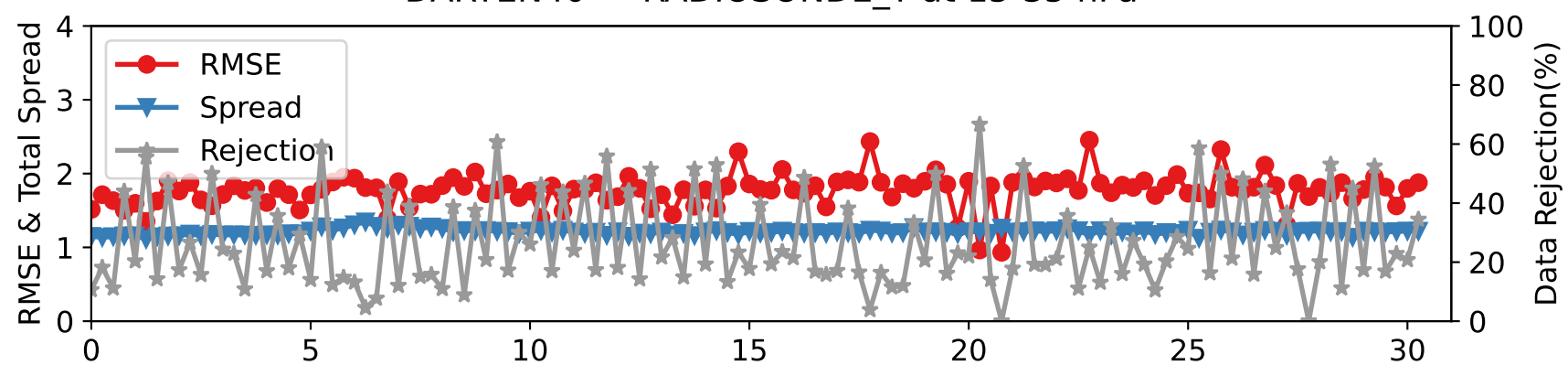
DARTEN40 — RADIOSONDE_T at 15-35 hPa
