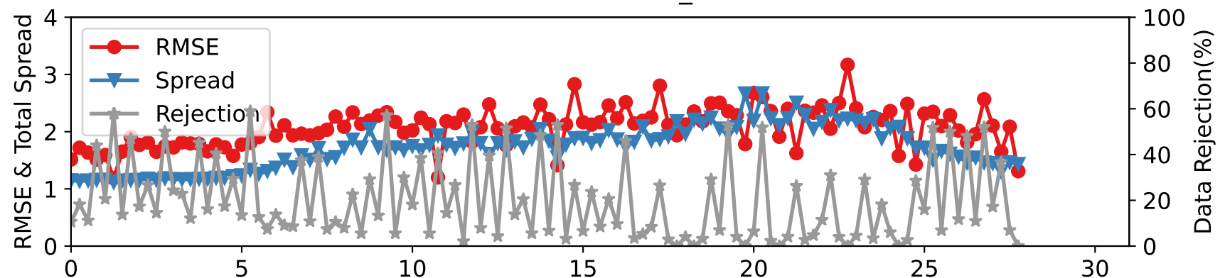
DARTEN10 — RADIOSONDE_T at 15-35 hPa
