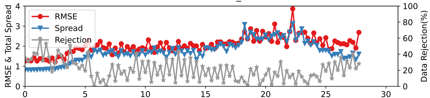
DARTEN10 — RADIOSONDE_T at 75-125 hPa
