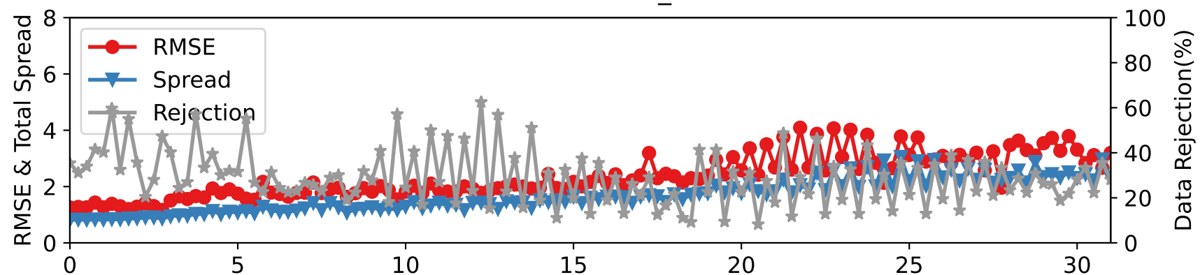
CTRLN10 — RADIOSONDE_T at 75-125 hPa
