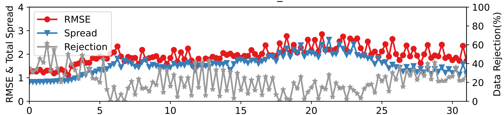
DARTEN20 — RADIOSONDE_T at 75-125 hPa
