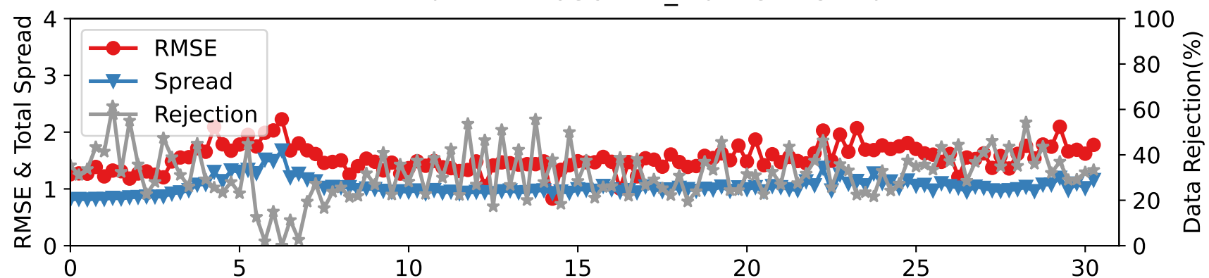
DARTEN40 — RADIOSONDE_T at 75-125 hPa
