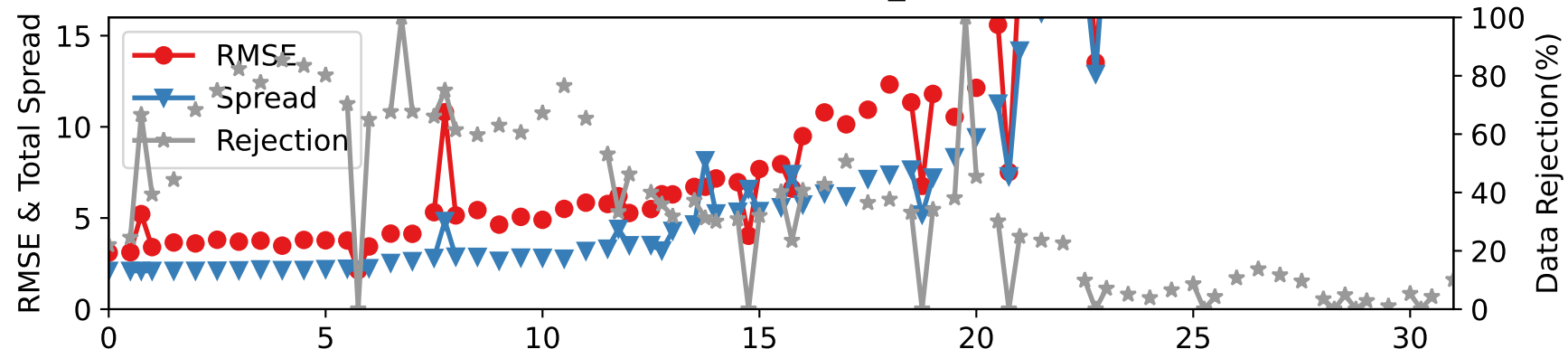
CTRLN10 — RADIOSONDE_U at 2-15 hPa
