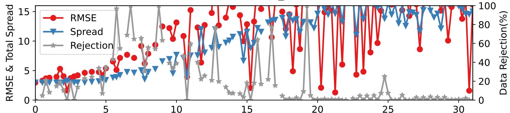
CTRLN10 — RADIOSONDE_U at 275-350 hPa
