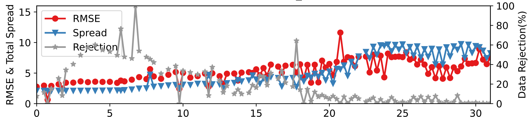
CTRLN10 — RADIOSONDE_U at 35-75 hPa
