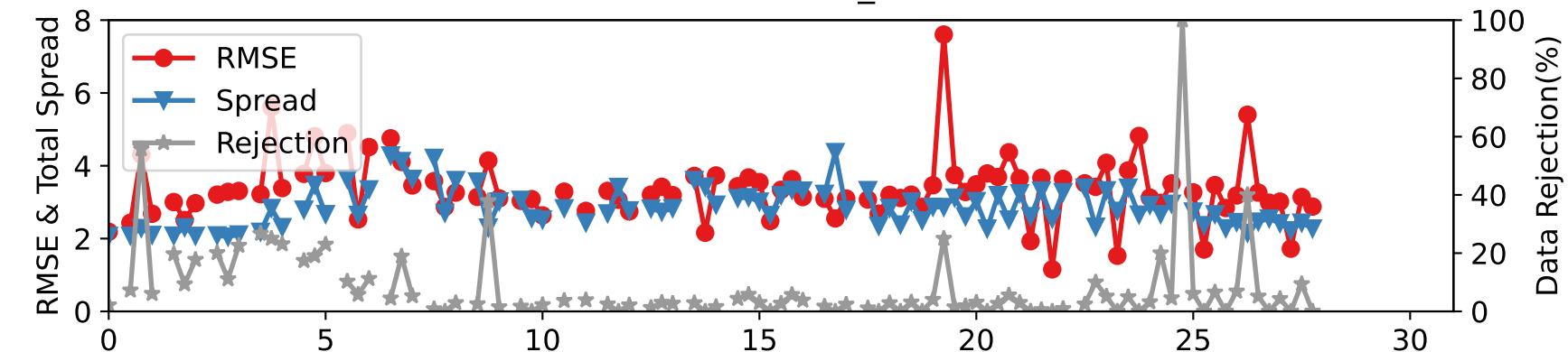
DARTEN10 — RADIOSONDE_U at 450-600 hPa
