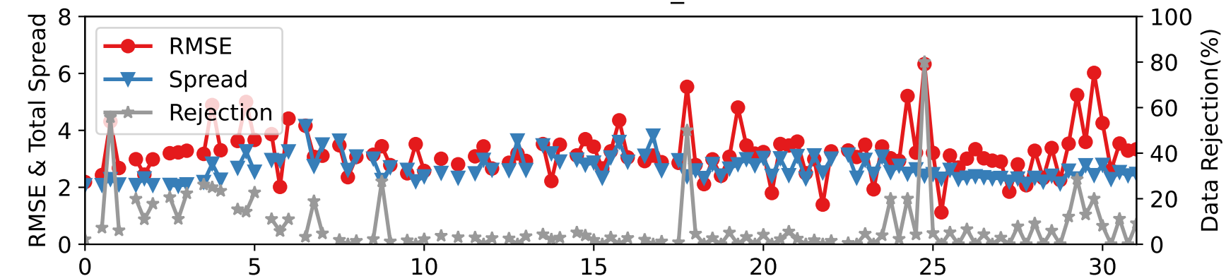
DARTEN20 — RADIOSONDE_U at 450-600 hPa
