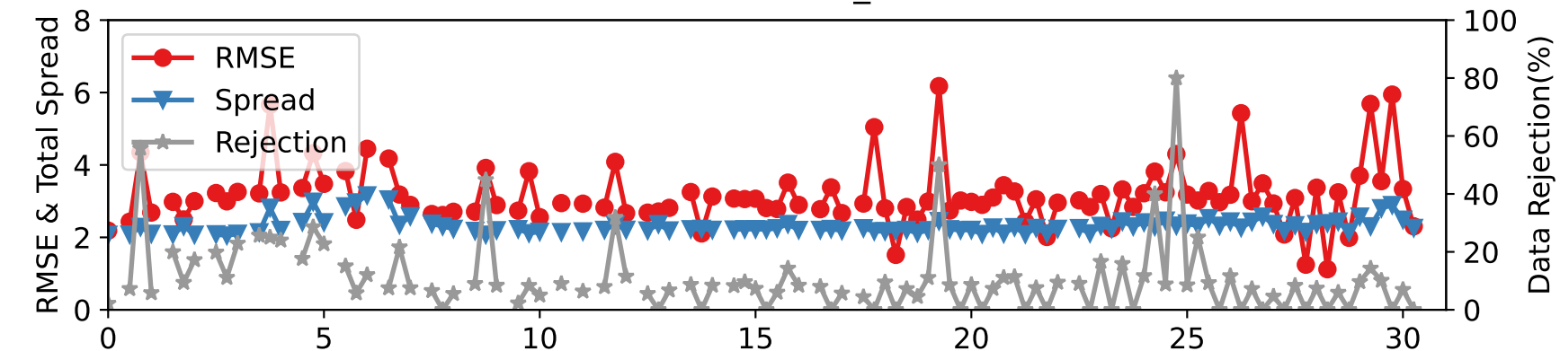
DARTEN40 — RADIOSONDE_U at 450-600 hPa
