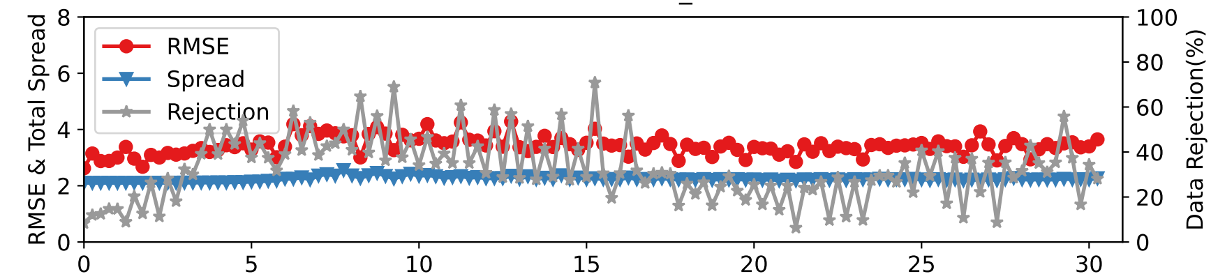
DARTEN40 — RADIOSONDE_U at 15-35 hPa
