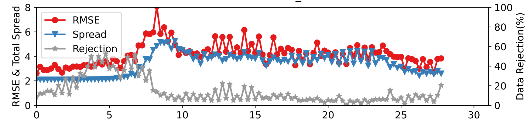
DARTEN10 — RADIOSONDE_U at 15-35 hPa
