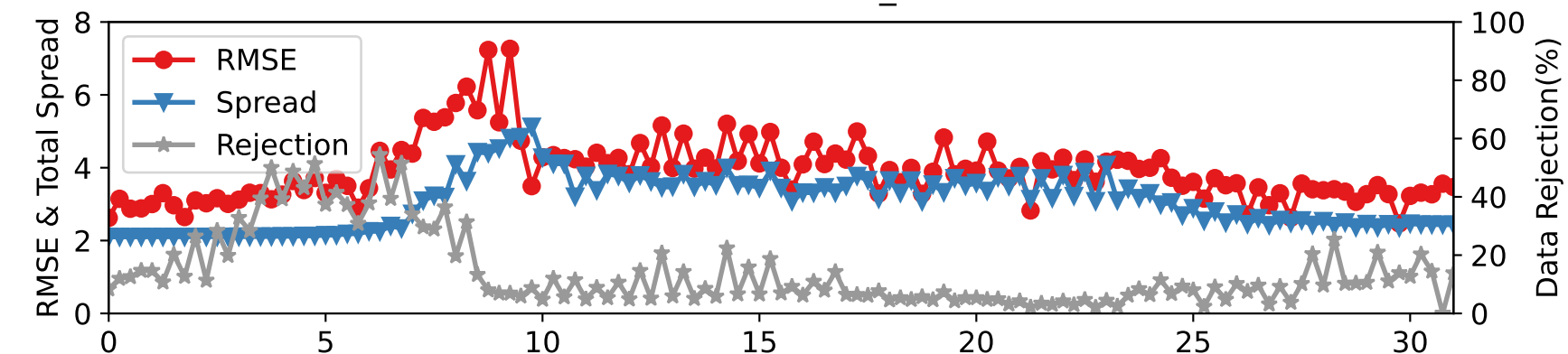
DARTEN20 — RADIOSONDE_U at 15-35 hPa
