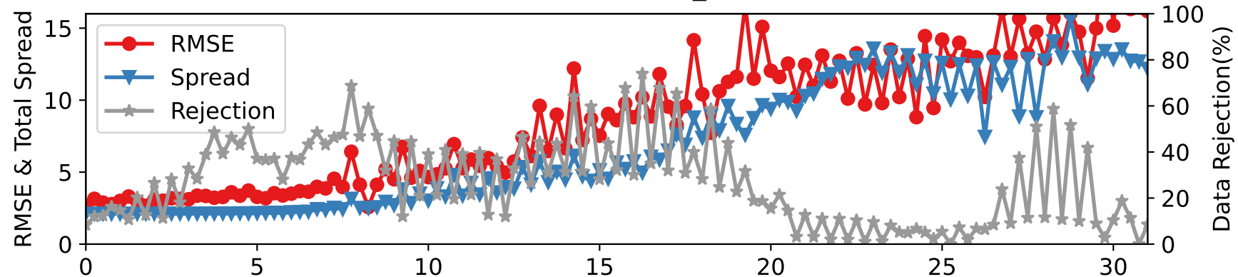
CTRLN10 — RADIOSONDE_U at 15-35 hPa
